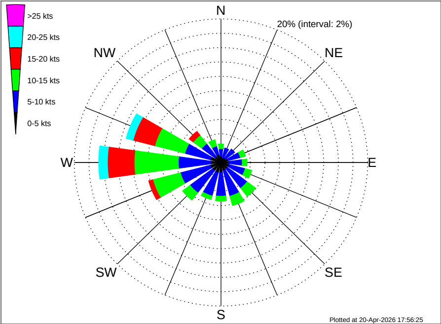
Petronas Oman Block 18 Climatological Wind Rose for February: 1979 - 2015
