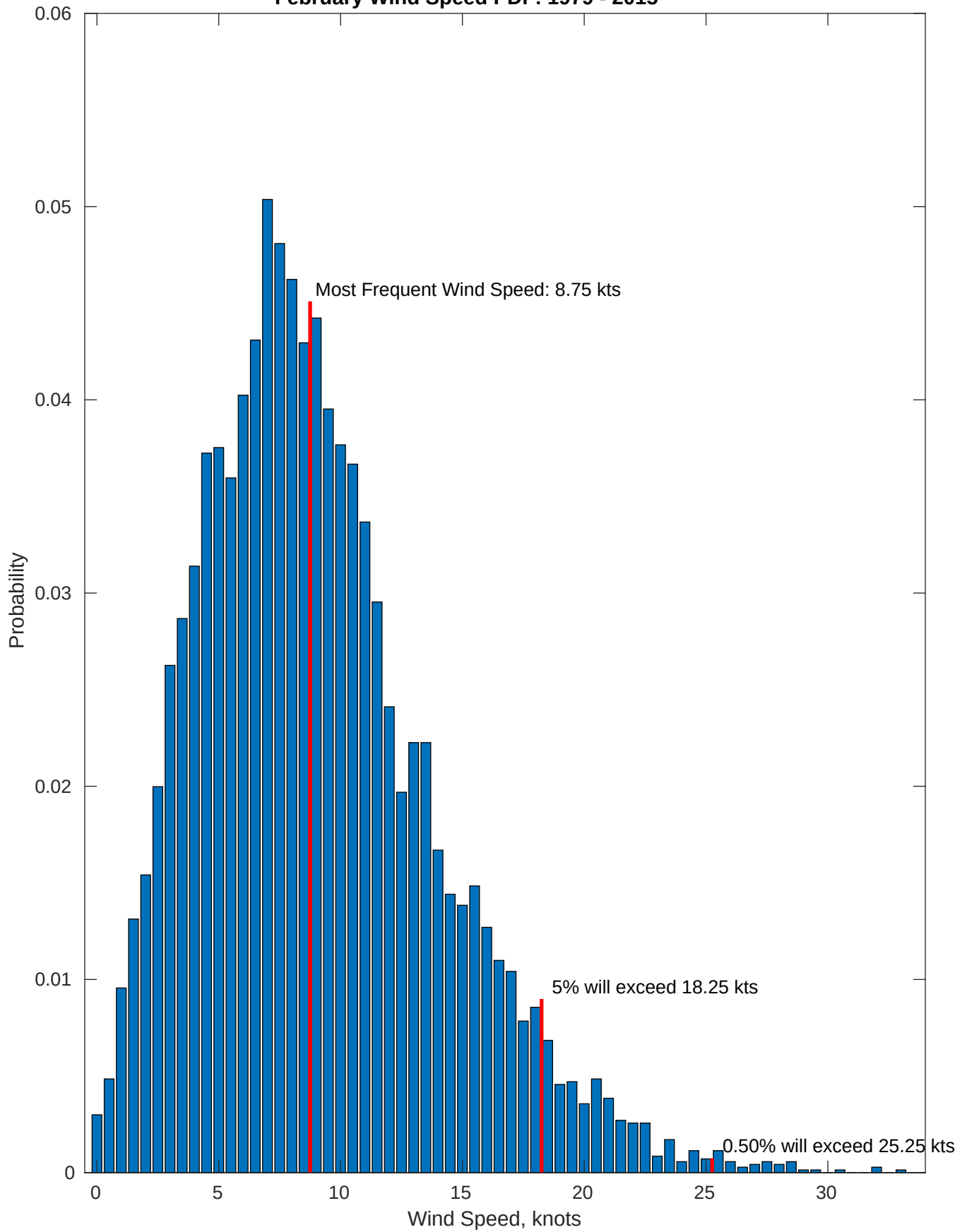
February Wind Speed PDF: 1979 - 2015
