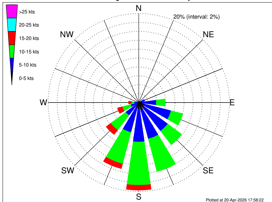
Petronas Oman Block 18 Climatological Wind Rose for July: 1979 - 2015
