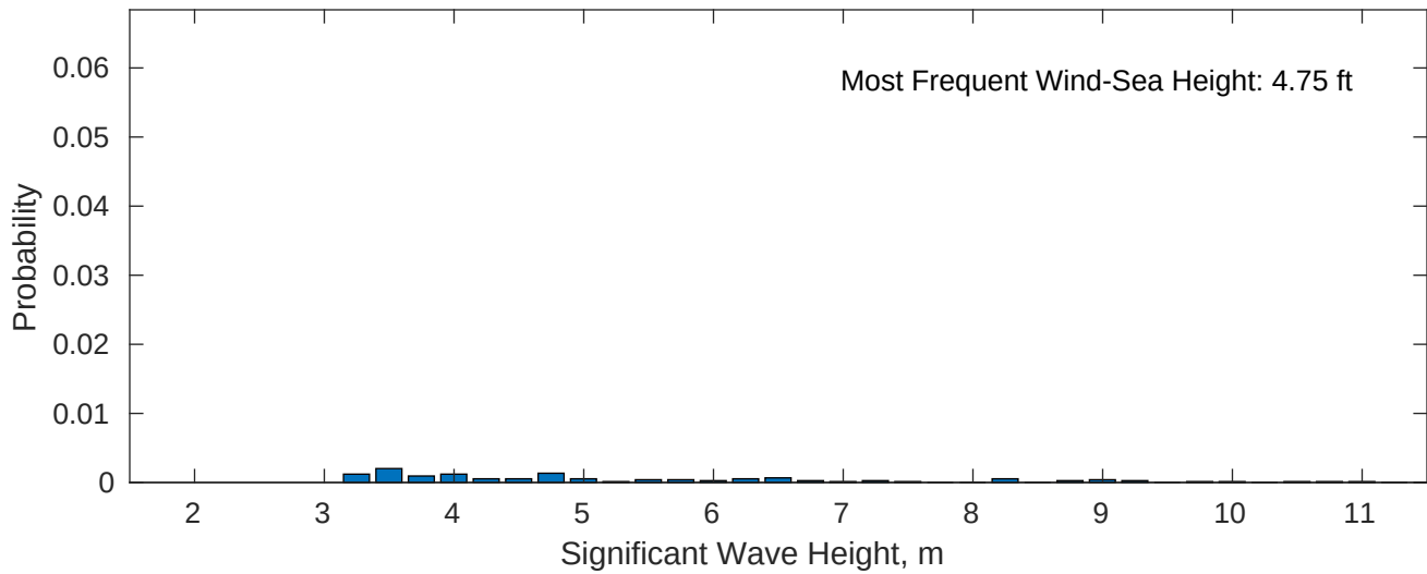
Wind-Sea: 1.37%
