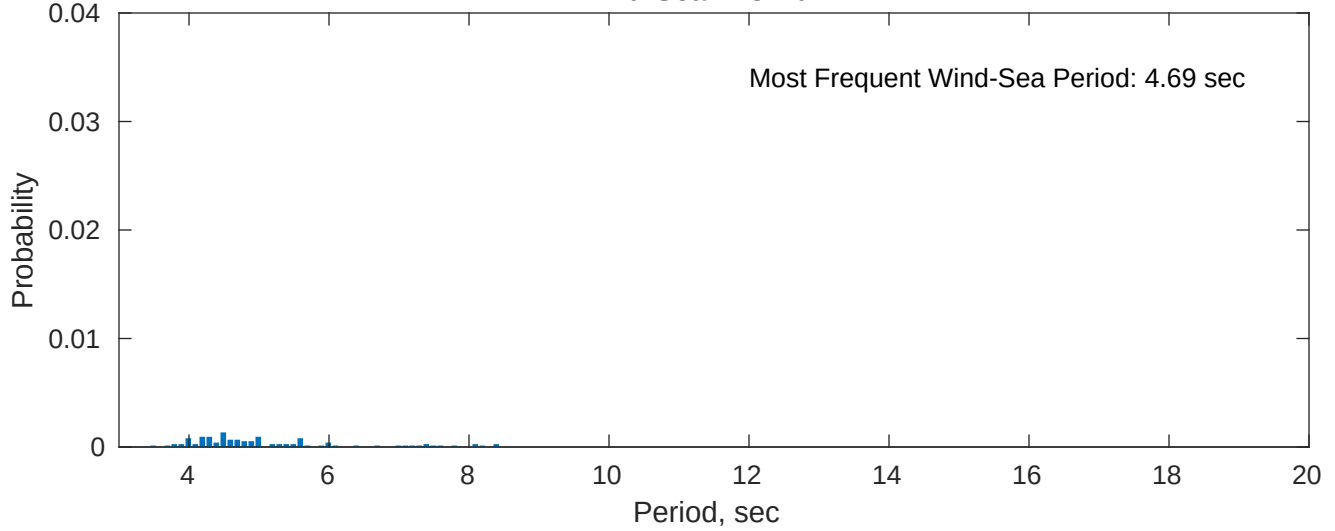
Wind-Sea: 1.37%
