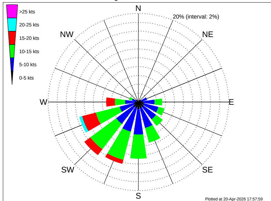
Petronas Oman Block 18 Climatological Wind Rose for June: 1979 - 2015
