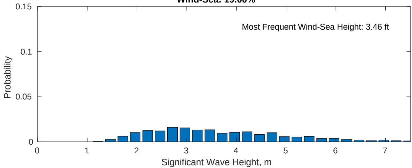
Wind-Sea: 19.00%
