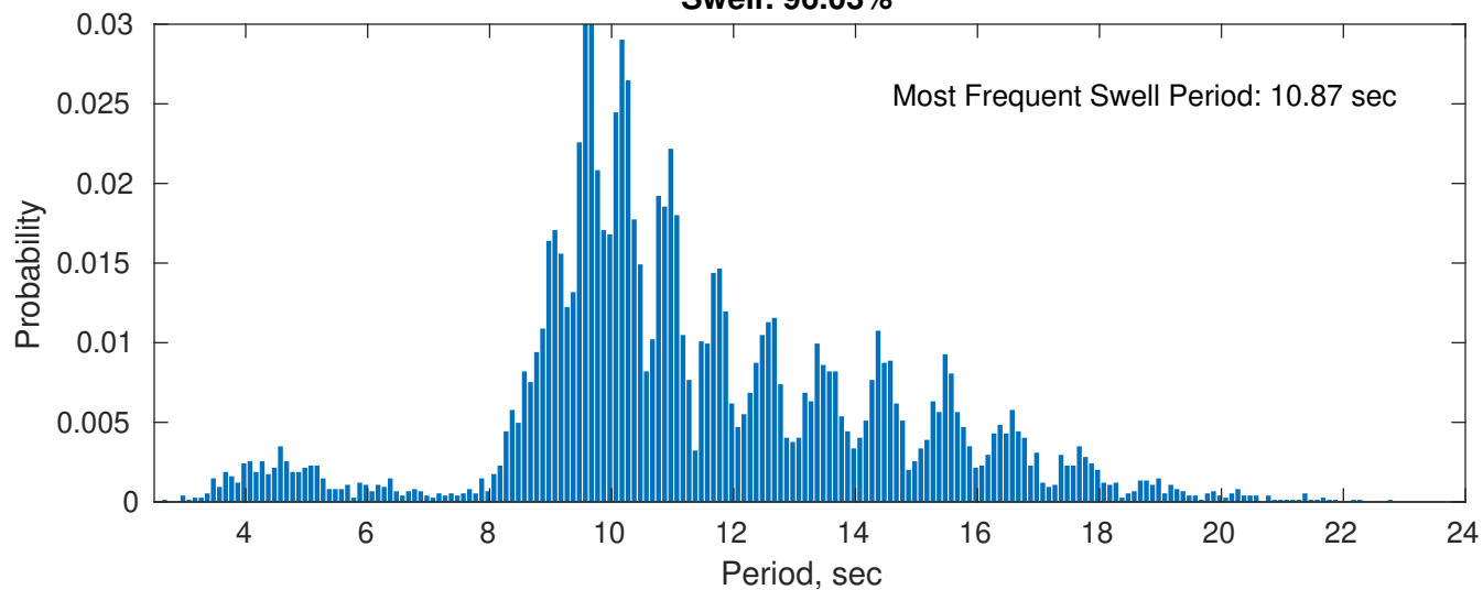
Swell: 96.03%
