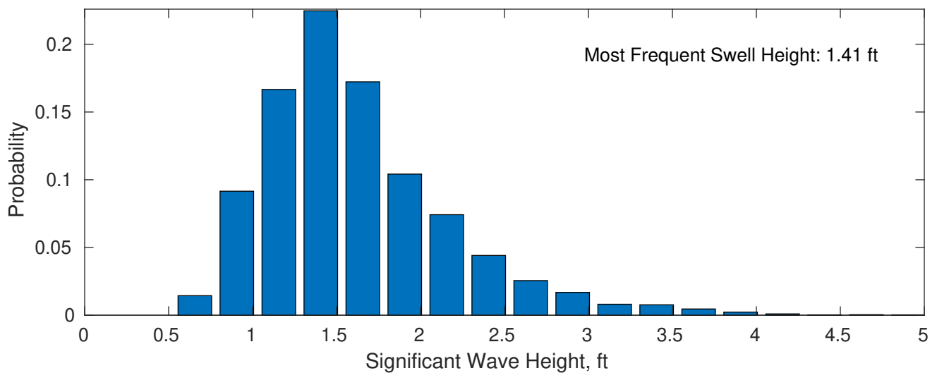
Swell: 96.03%
