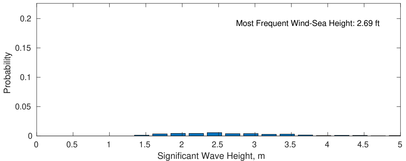
Wind-Sea: 3.97%
