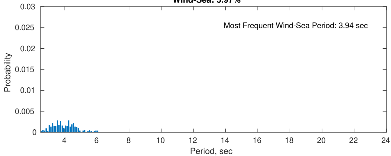
Wind-Sea: 3.97%
