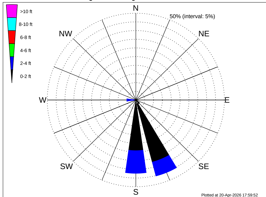
Petronas Oman Block 18 Climatological WaveHeight Rose for November: 1979 - 2015
