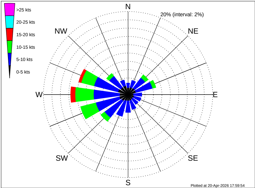
Petronas Oman Block 18 Climatological Wind Rose for November: 1979 - 2015
