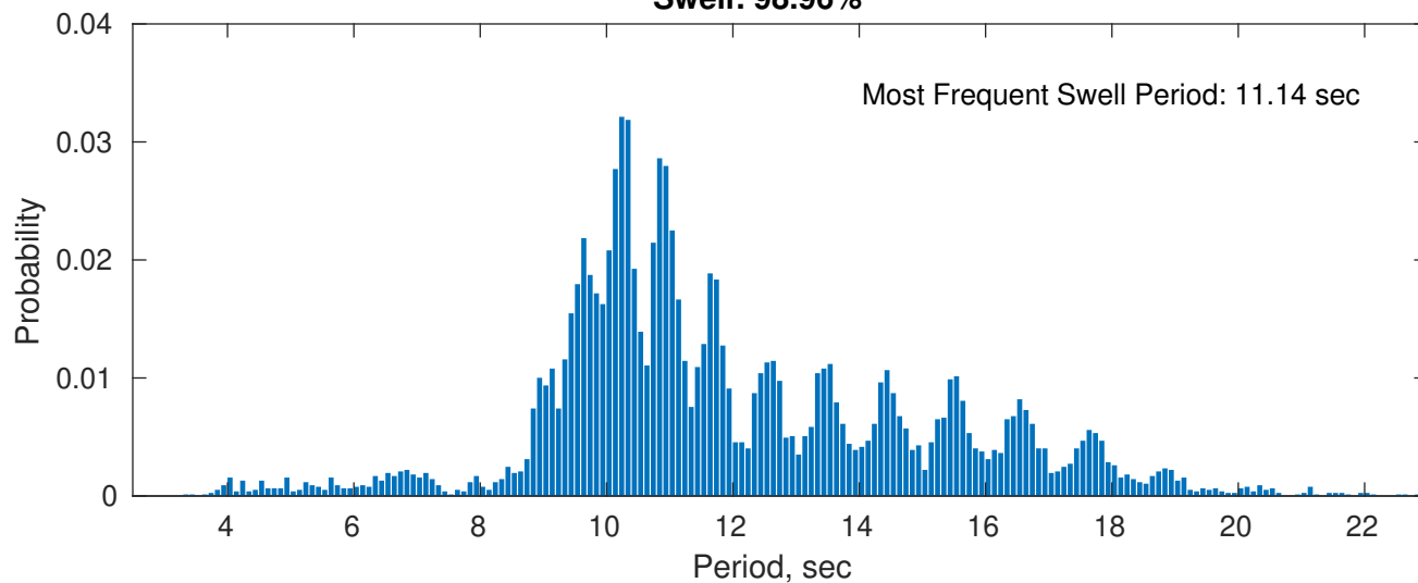
Swell: 98.96%
