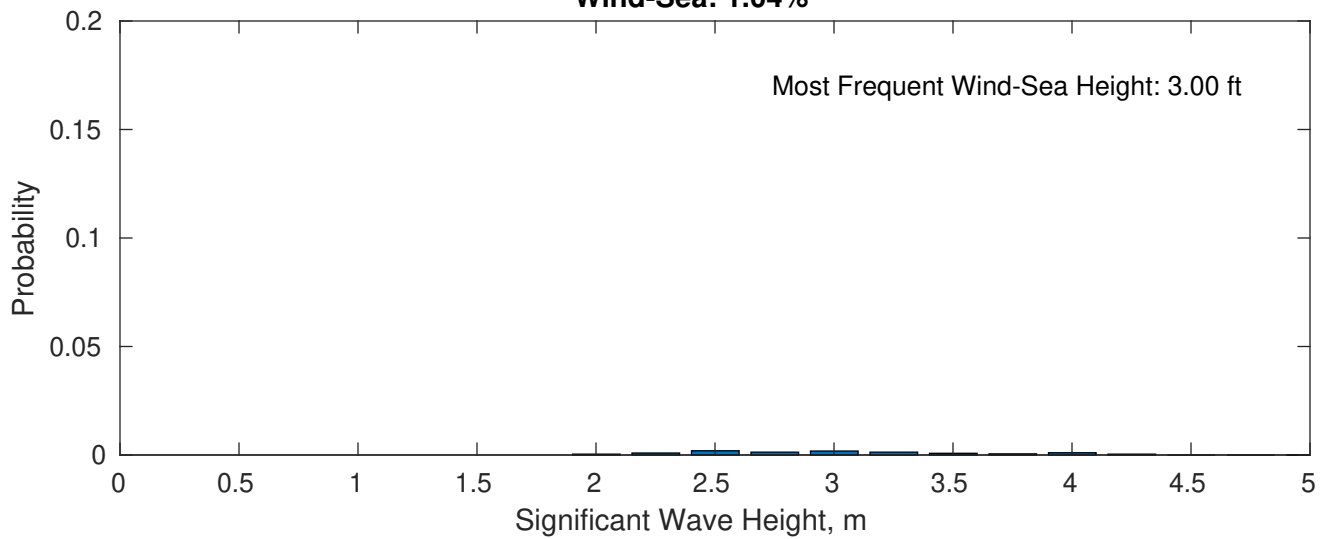
Wind-Sea: 1.04%
