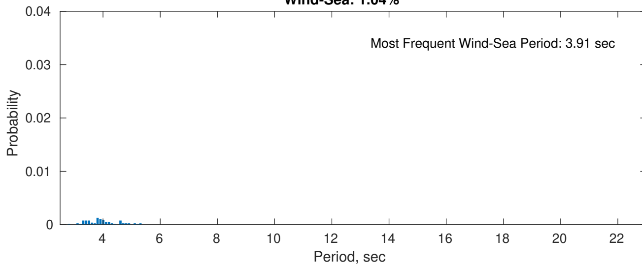
Wind-Sea: 1.04%
