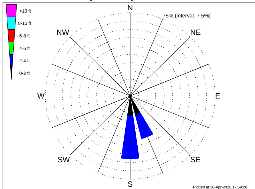
Petronas Oman Block 18 Climatological WaveHeight Rose for October: 1979 - 2015
