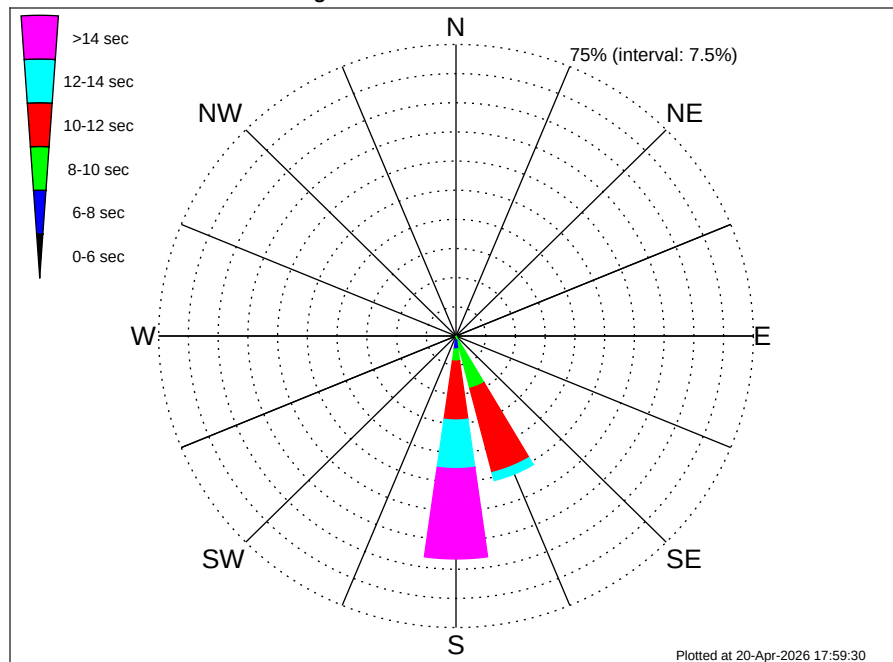
Petronas Oman Block 18 Climatological WavePeriod Rose for October: 1979 - 2015
