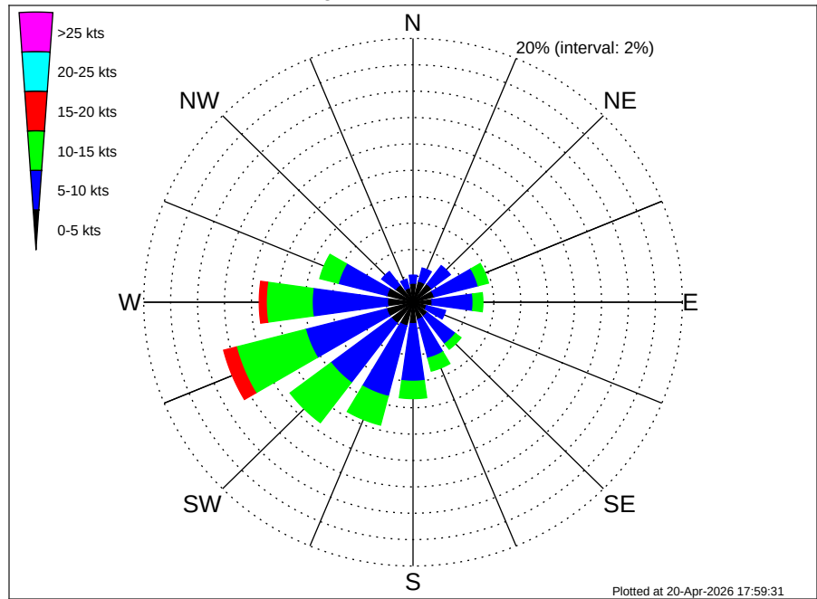
Petronas Oman Block 18 Climatological Wind Rose for October: 1979 - 2015
