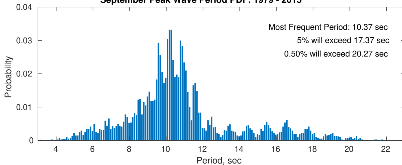
September Peak Wave Period PDF: 1979 - 2015
