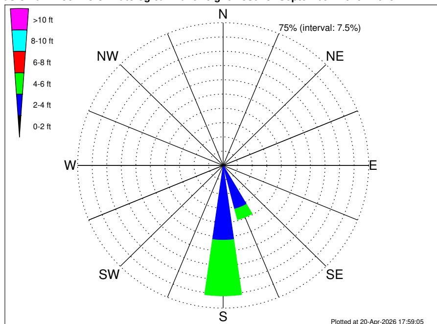
Petronas Oman Block 18 Climatological WaveHeight Rose for September: 1979 - 2015
