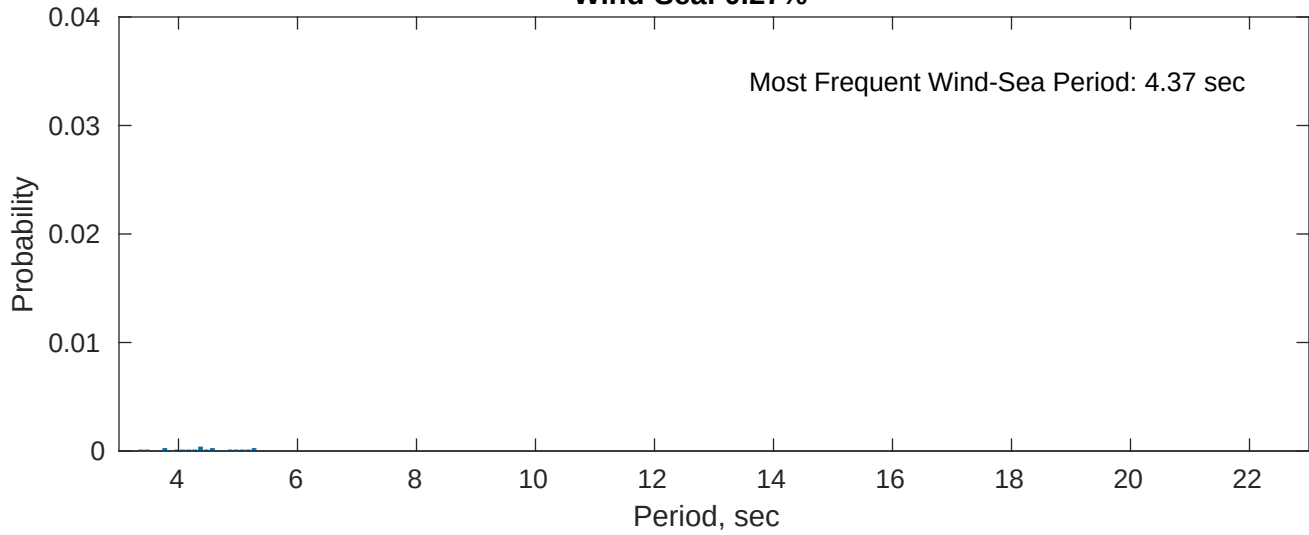
Wind-Sea: 0.27%
