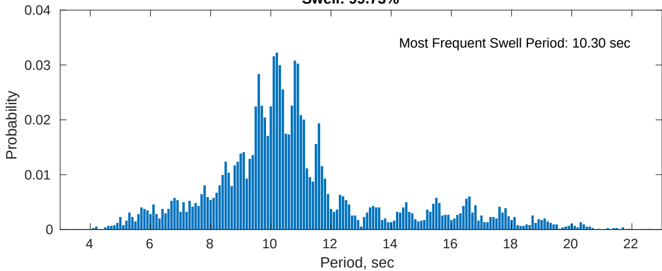
Swell: 99.73%
