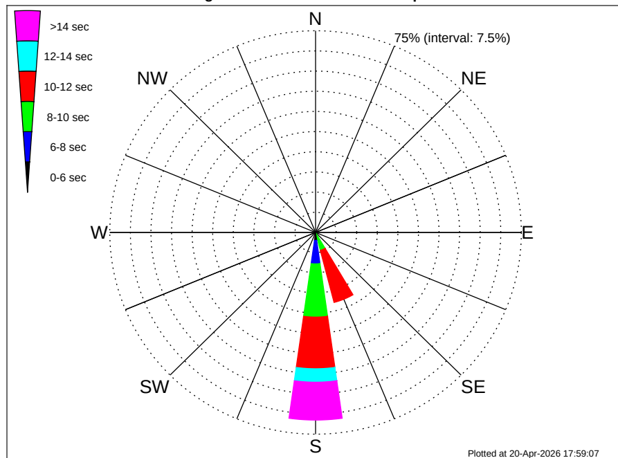
Petronas Oman Block 18 Climatological WavePeriod Rose for September: 1979 - 2015
