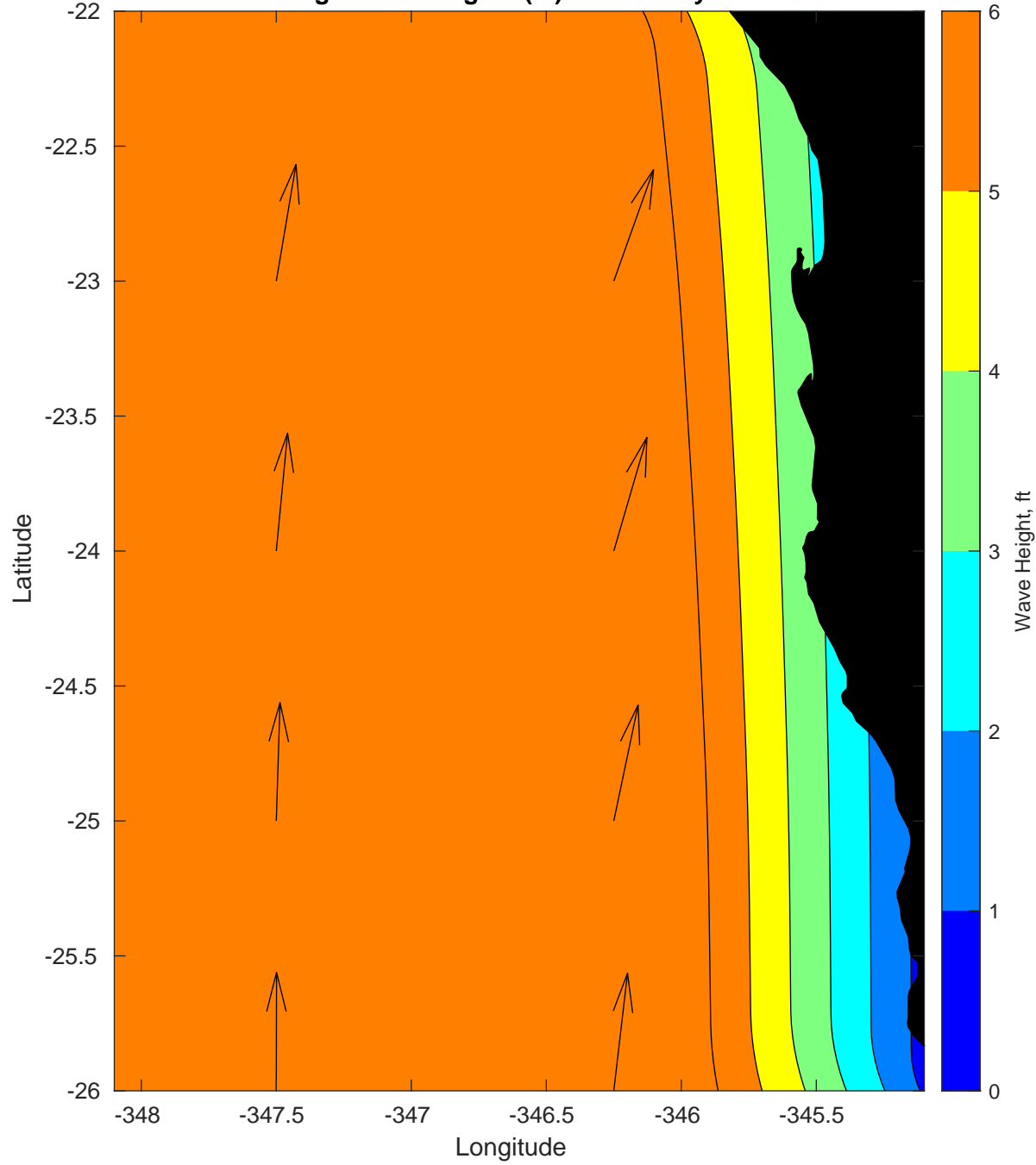
Average Wave Heights (m) for January
