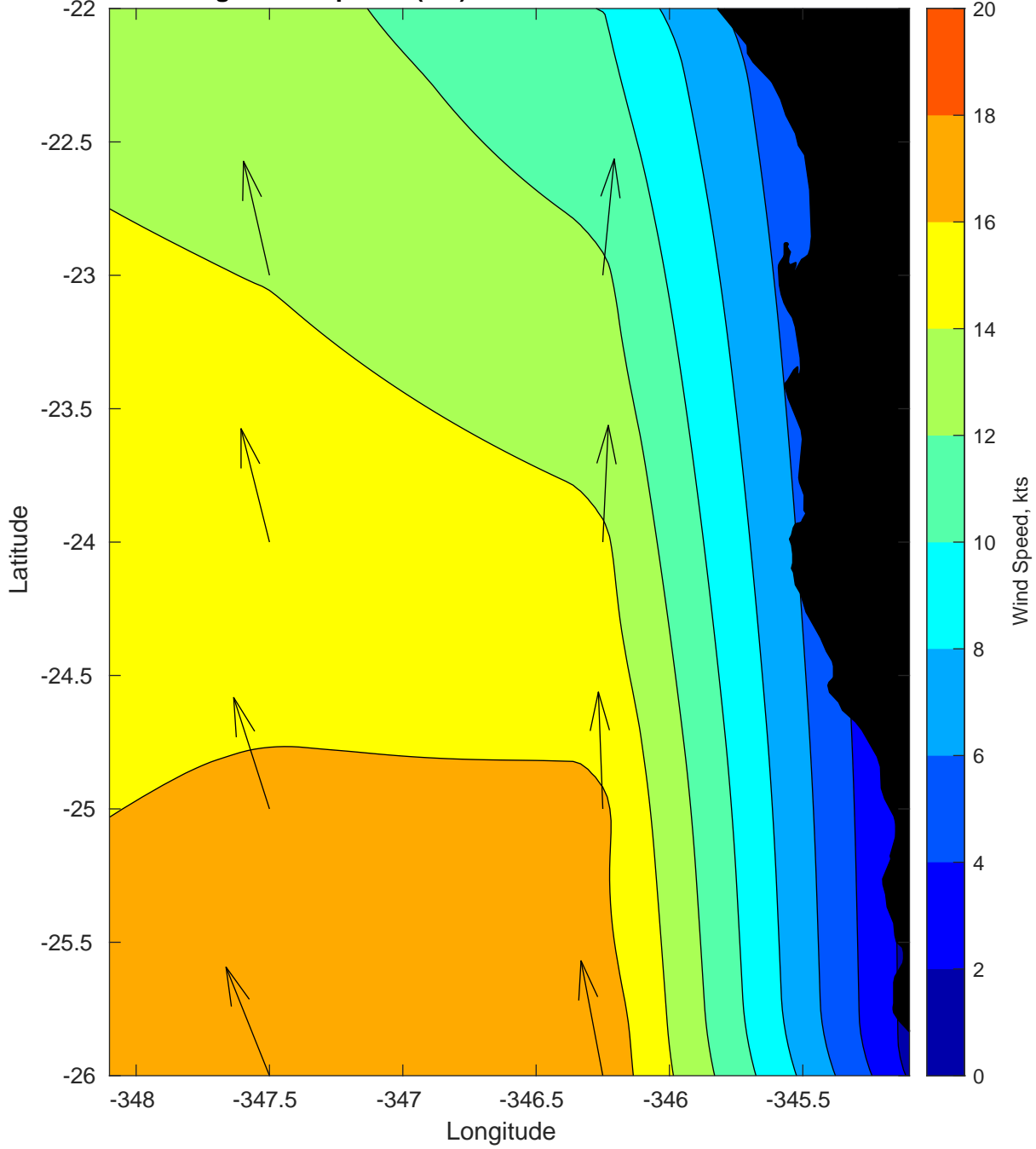
Average Wind Speeds (kts) and Direction for March
