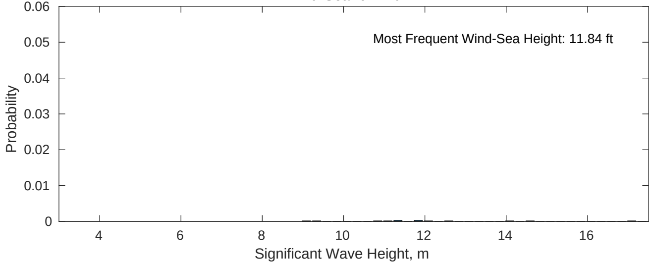
Wind-Sea: 0.17%
