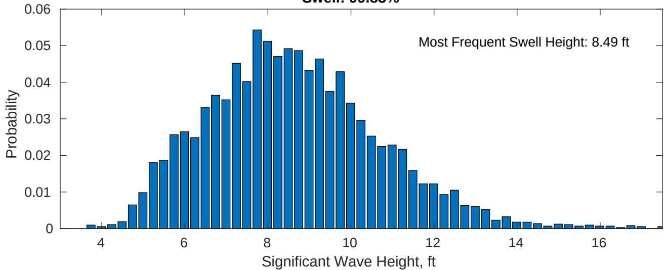
Swell: 99.83%
