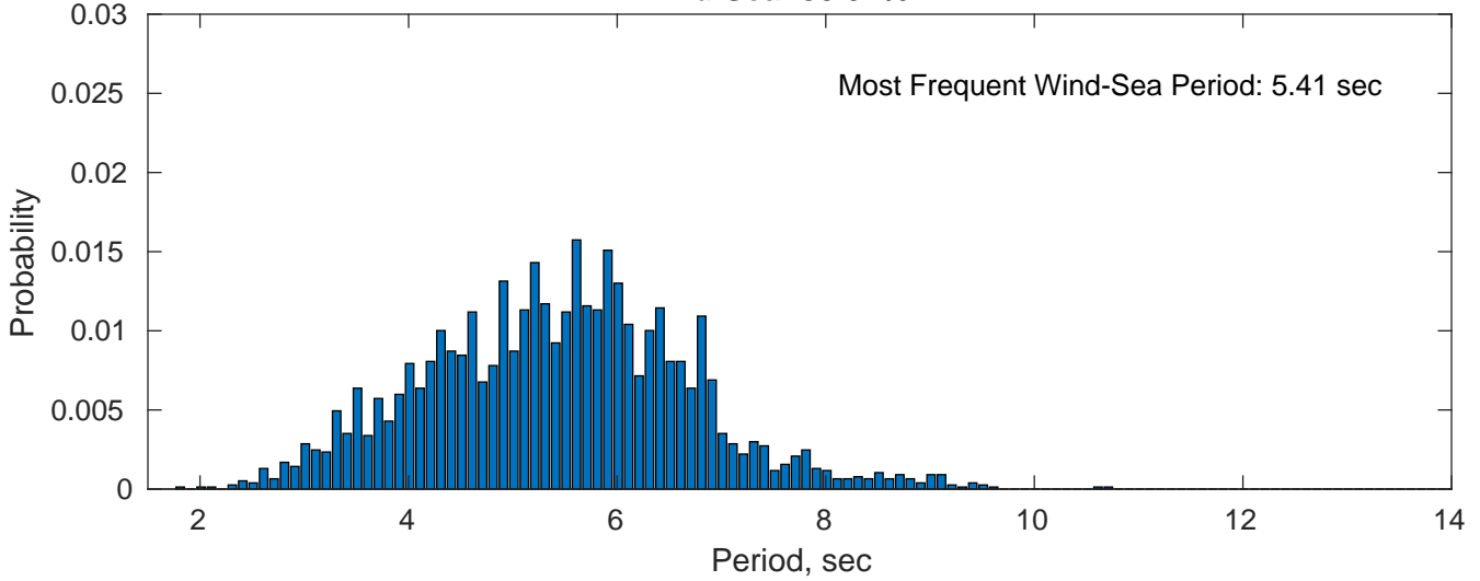
Wind-Sea: 38.32%
