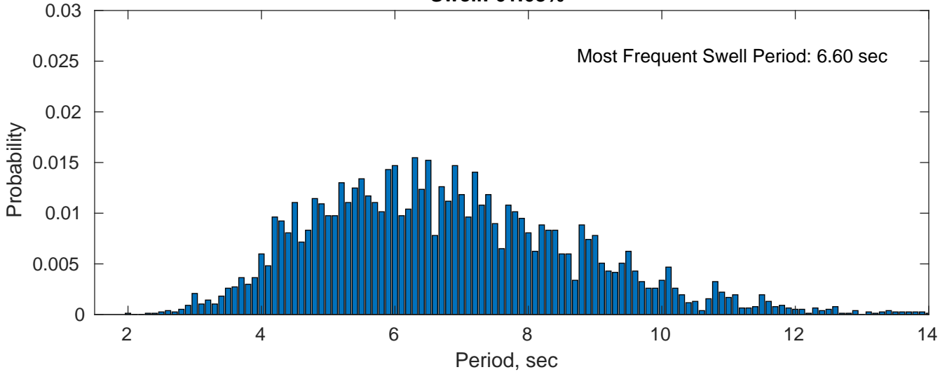
Swell: 61.68%
