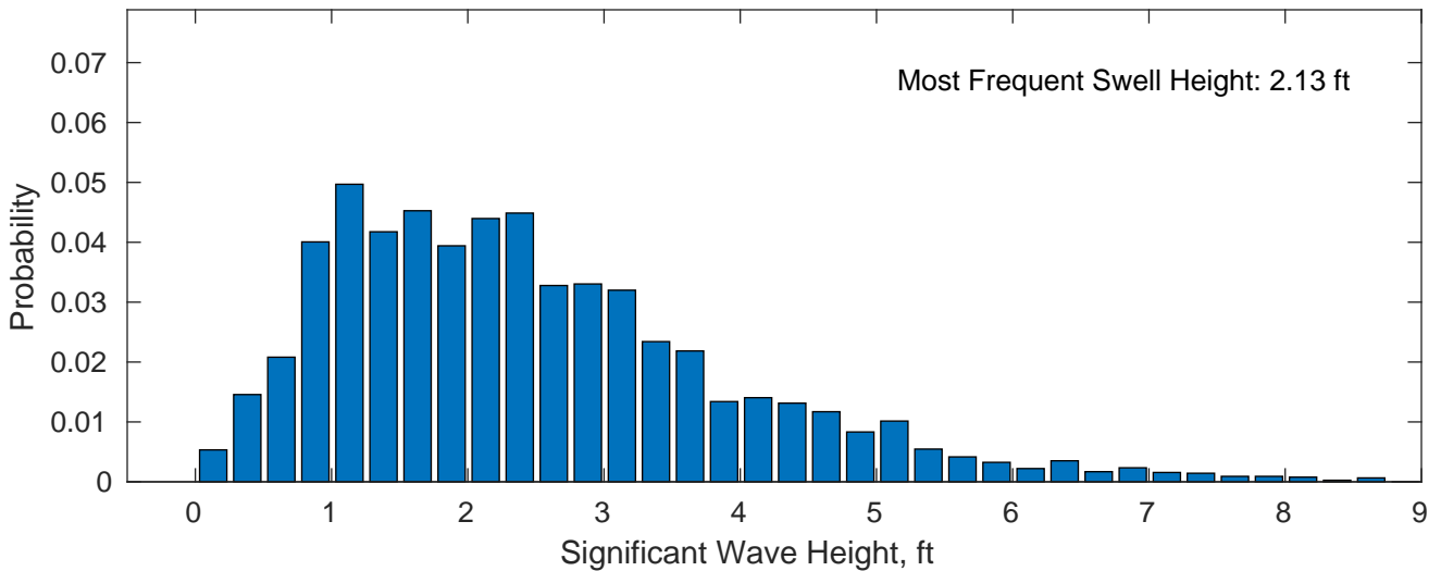
Swell: 58.94%
