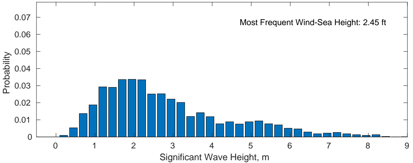
Wind-Sea: 41.06%
