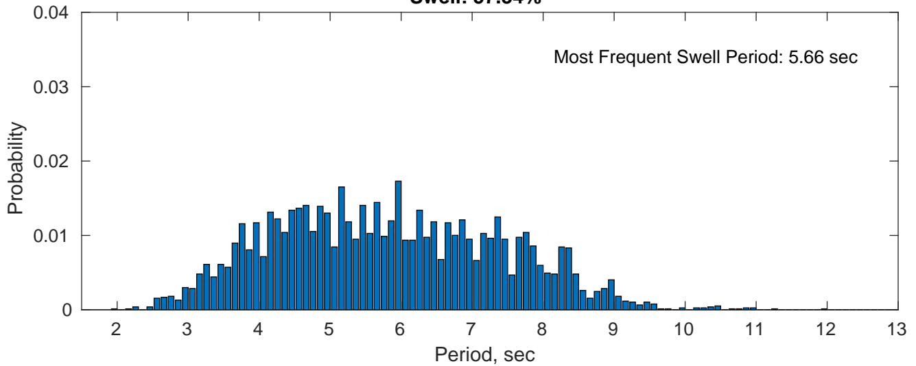
Swell: 57.34%
