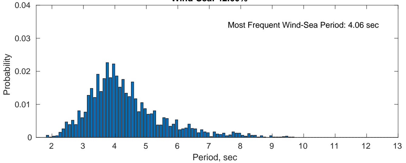
Wind-Sea: 42.66%
