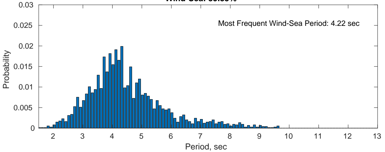
Wind-Sea: 39.33%
