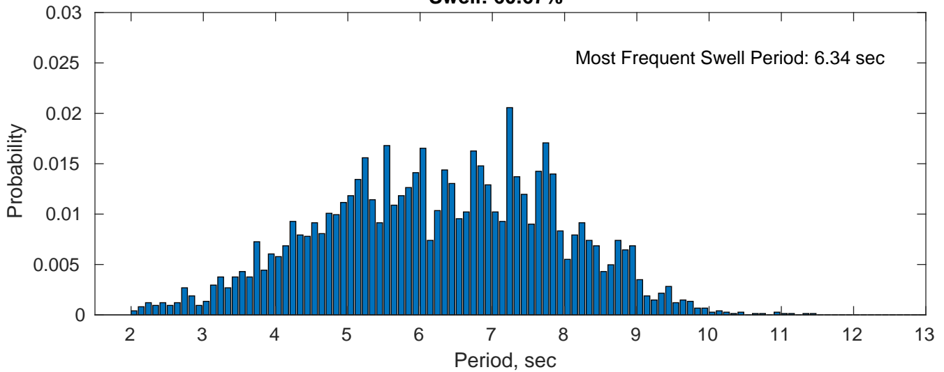
Swell: 60.67%
