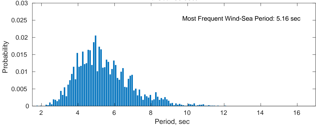
Wind-Sea: 50.98%
