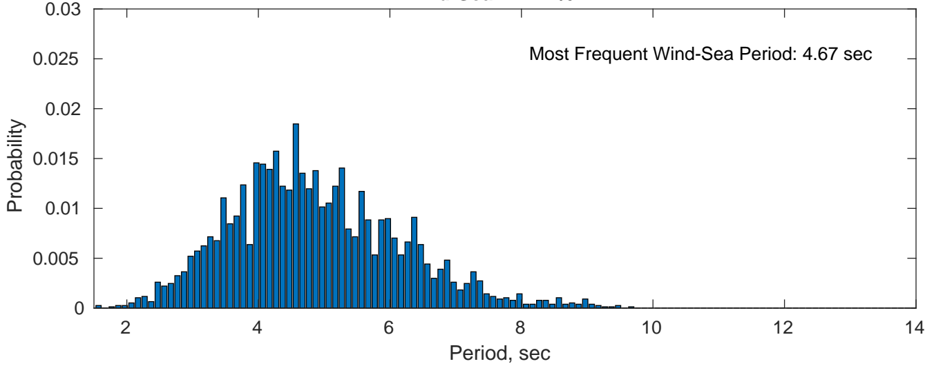
Wind-Sea: 42.12%
