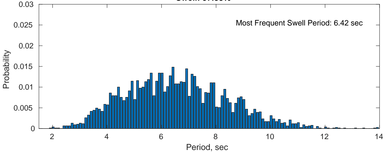
Swell: 57.88%
