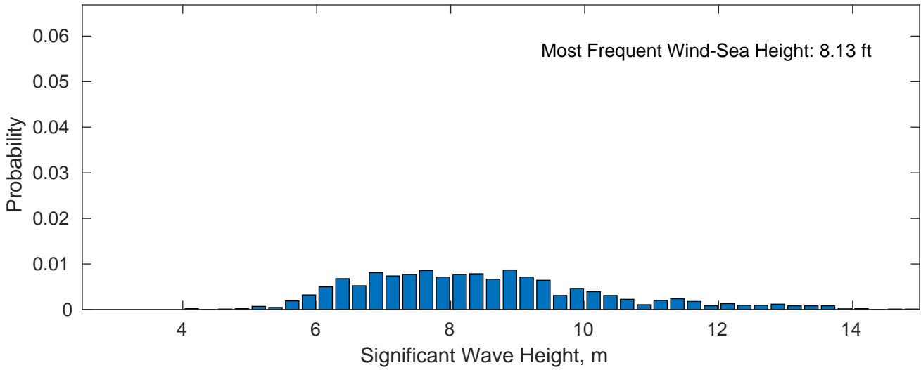
Wind-Sea: 14.03%
