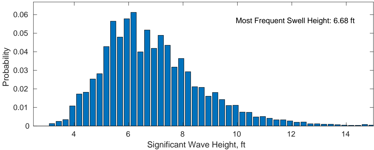
Swell: 85.97%
