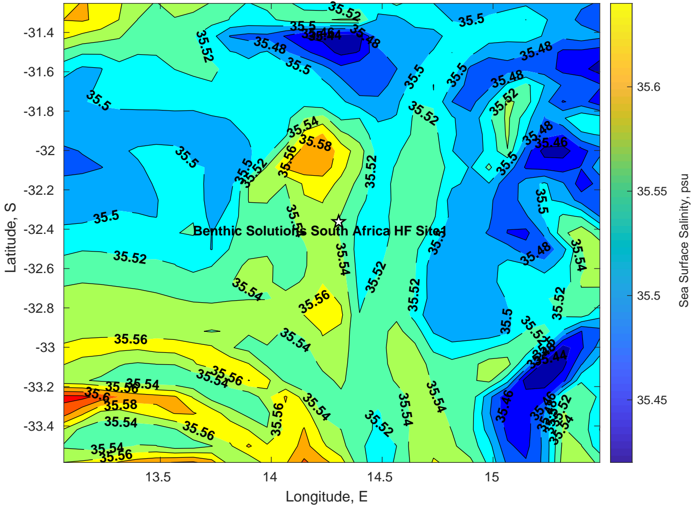
Surface Salinity for Benthic Solutions South Africa HF Site1 at 10-Apr-2025 00:00:00
