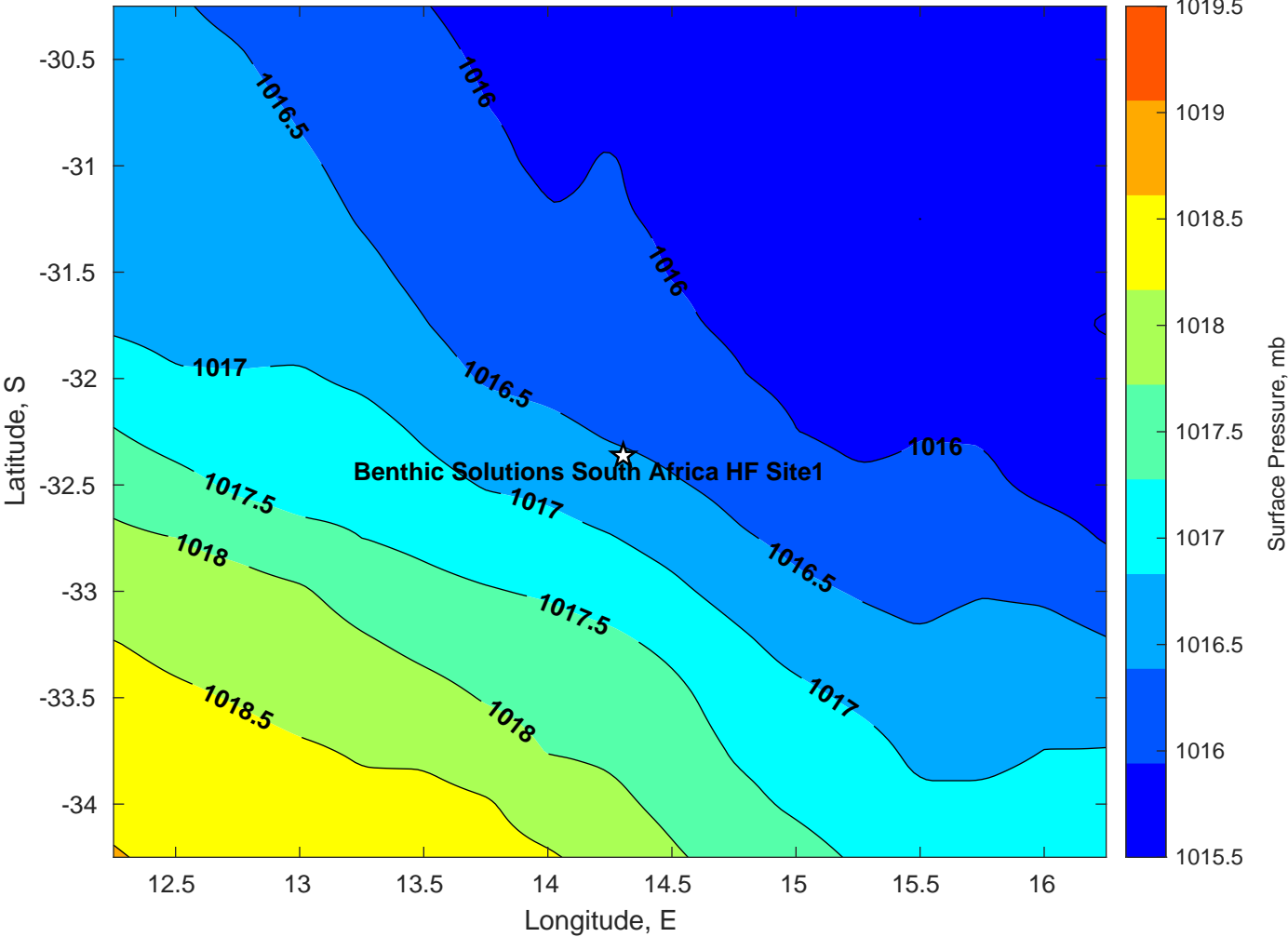
Surface Pressure (mb) for Benthic Solutions South Africa HF Site1 at 12-Apr-2025 12:00:00
