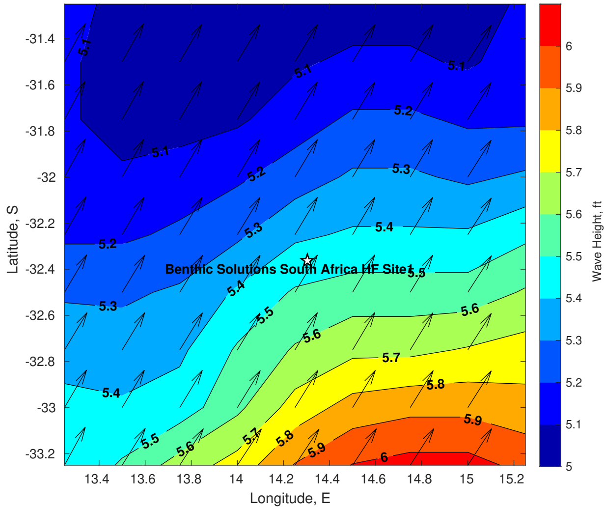
Wave Height (ft) for Benthic Solutions South Africa HF Site1 at 10-Apr-2025 21:00:00
