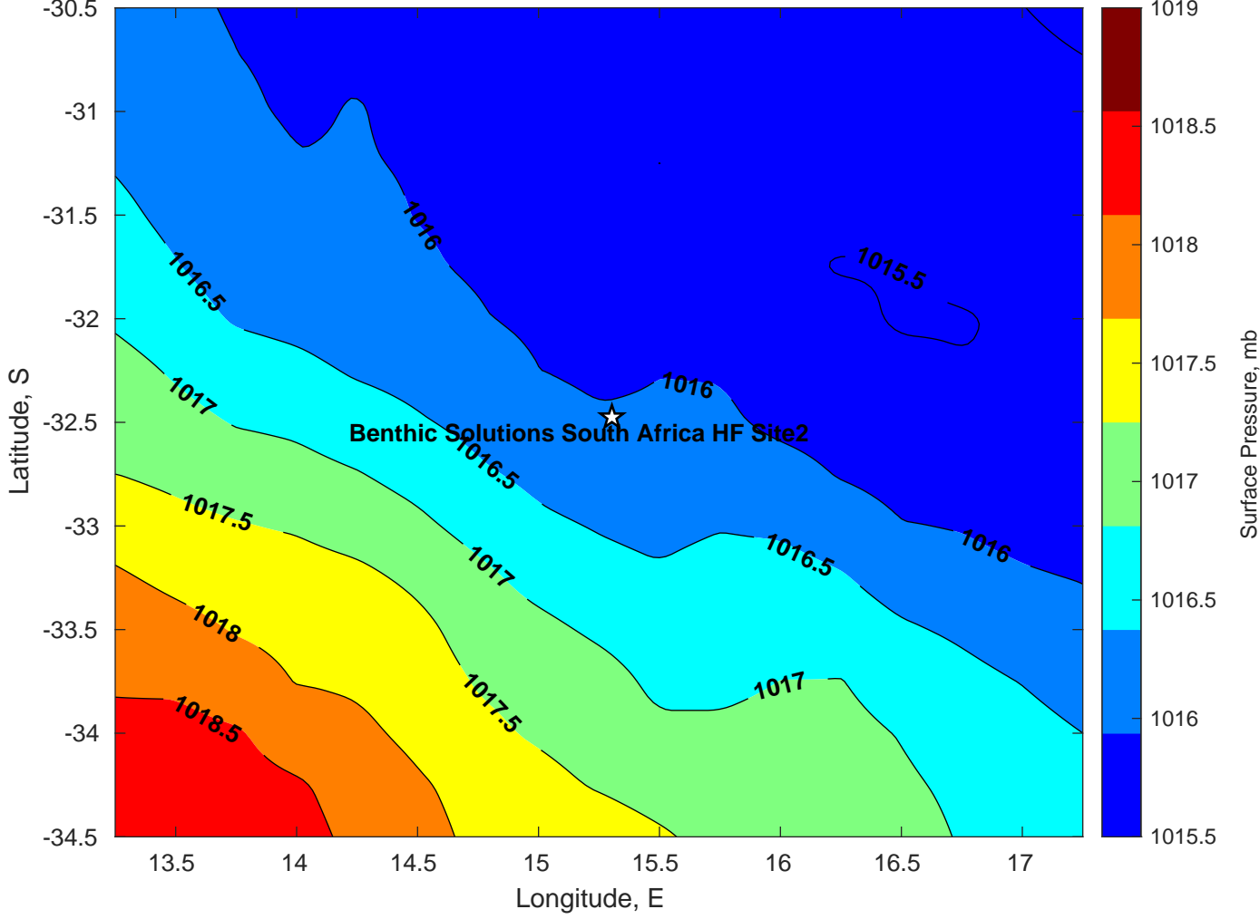
Surface Pressure (mb) for Benthic Solutions South Africa HF Site2 at 12-Apr-2025 12:00:00
