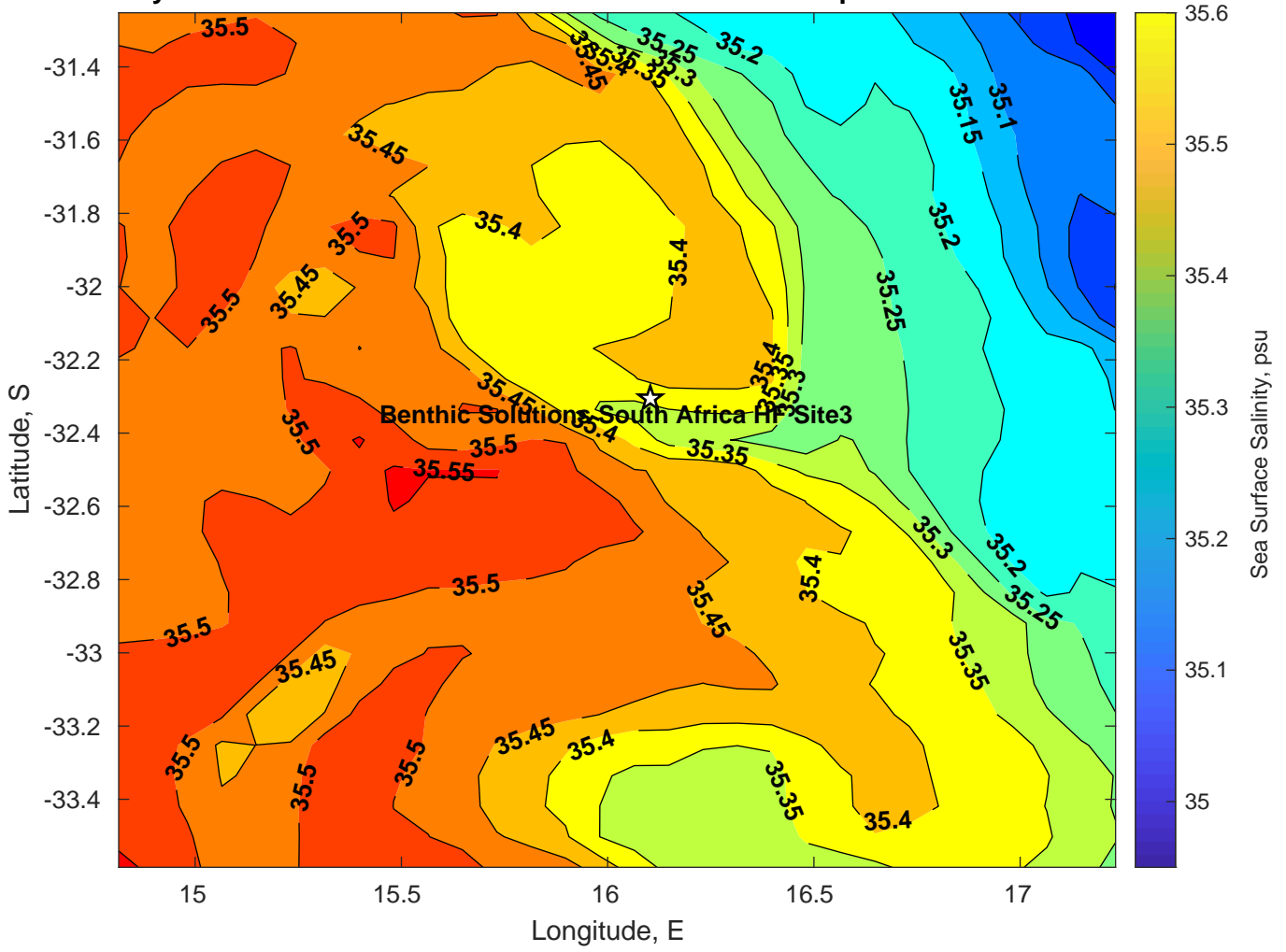
Surface Salinity for Benthic Solutions South Africa HF Site3 at 10-Apr-2025 00:00:00
