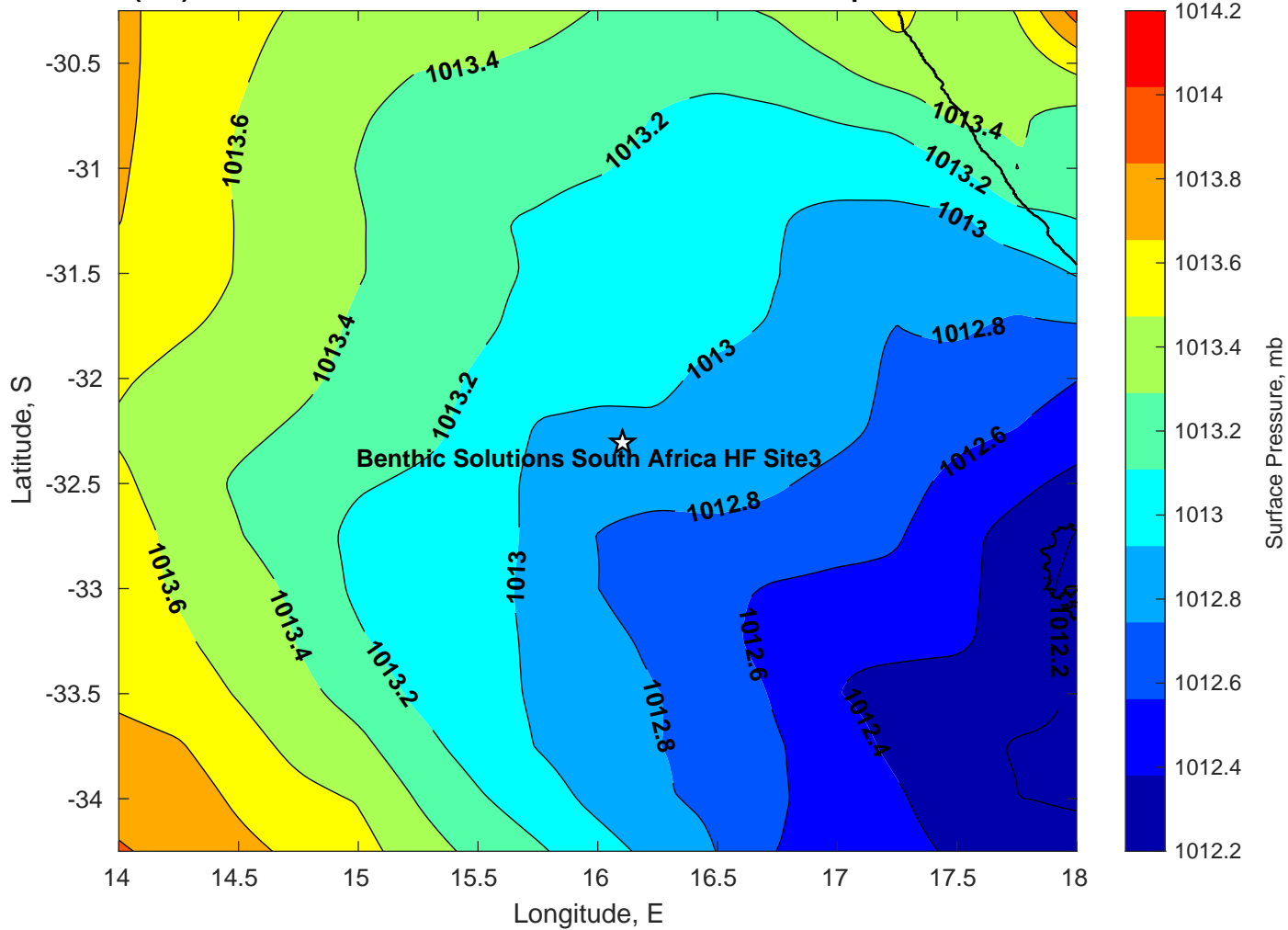
Surface Pressure (mb) for Benthic Solutions South Africa HF Site3 at 11-Apr-2025 00:00:00
