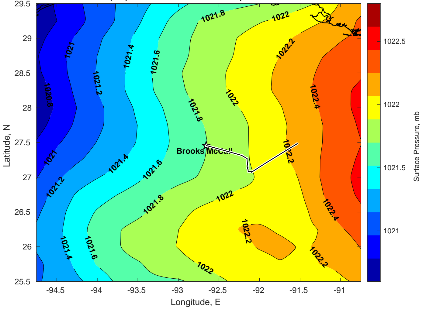
Surface Pressure (mb) for Brooks McCall at 10-Apr-2025 12:00:00
