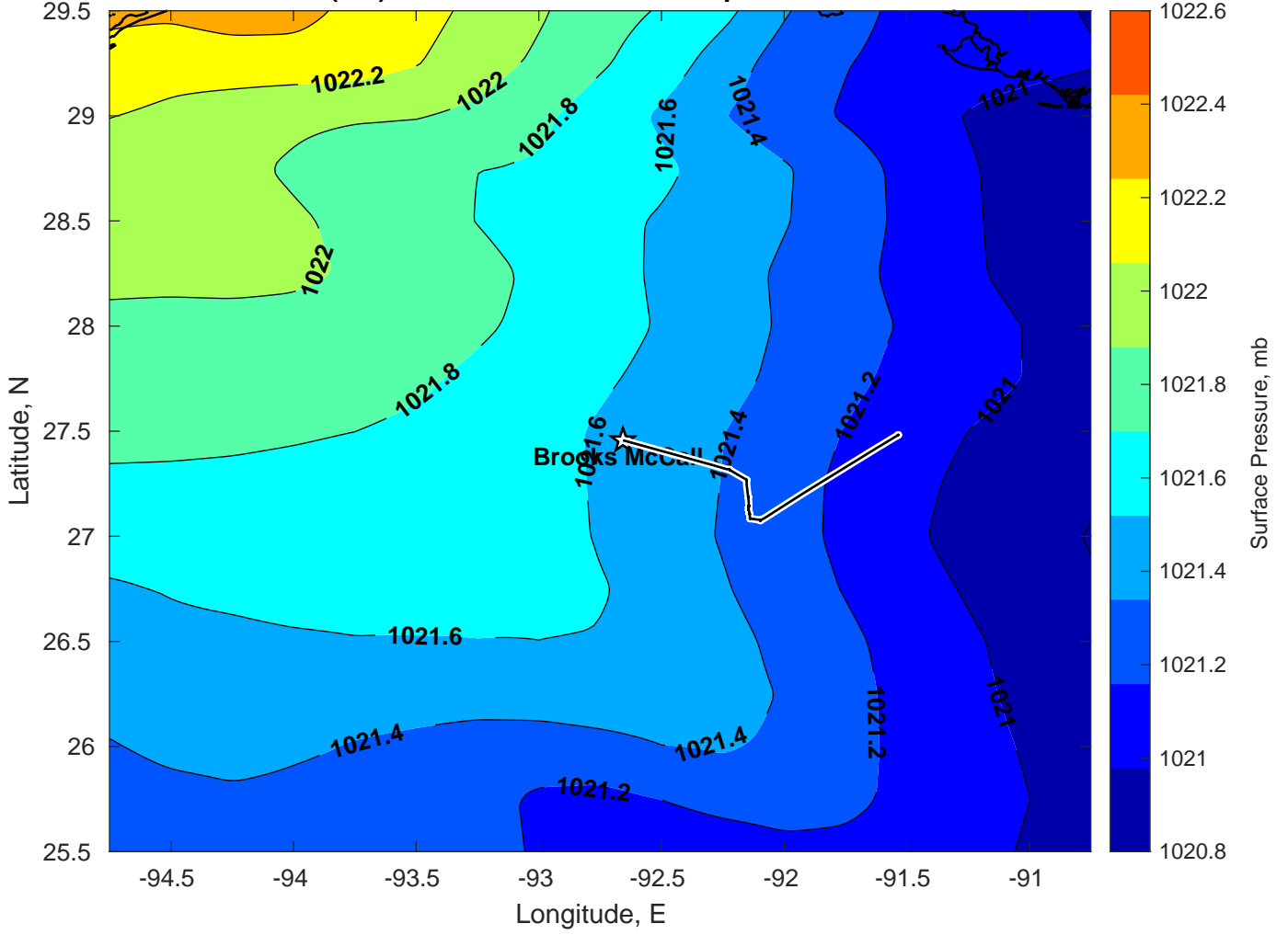
Surface Pressure (mb) for Brooks McCall at 11-Apr-2025 12:00:00
