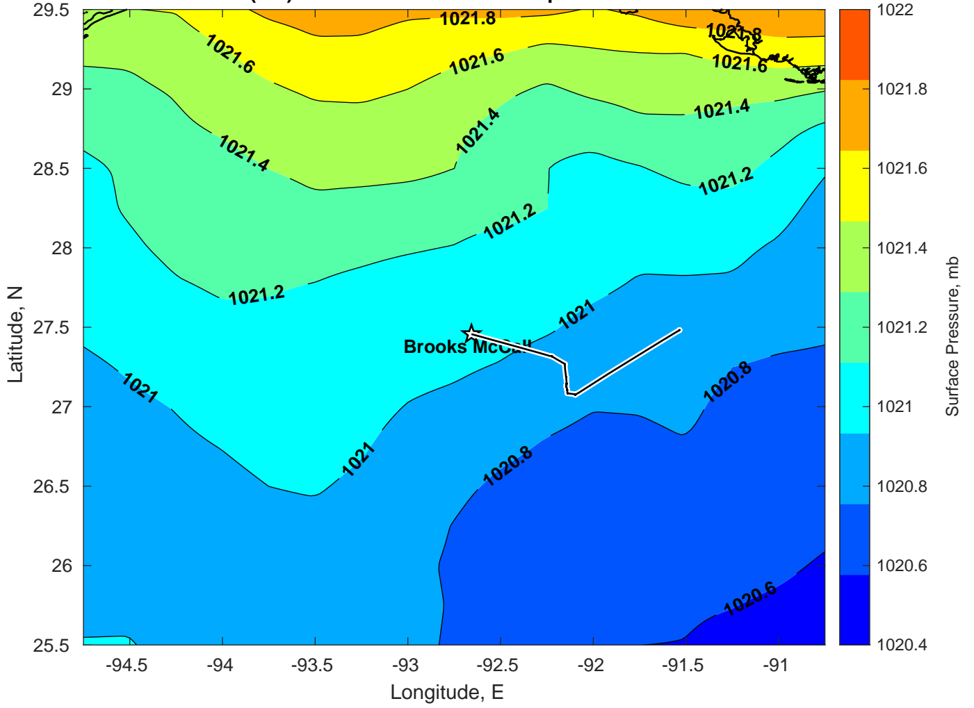
Surface Pressure (mb) for Brooks McCall at 12-Apr-2025 12:00:00
