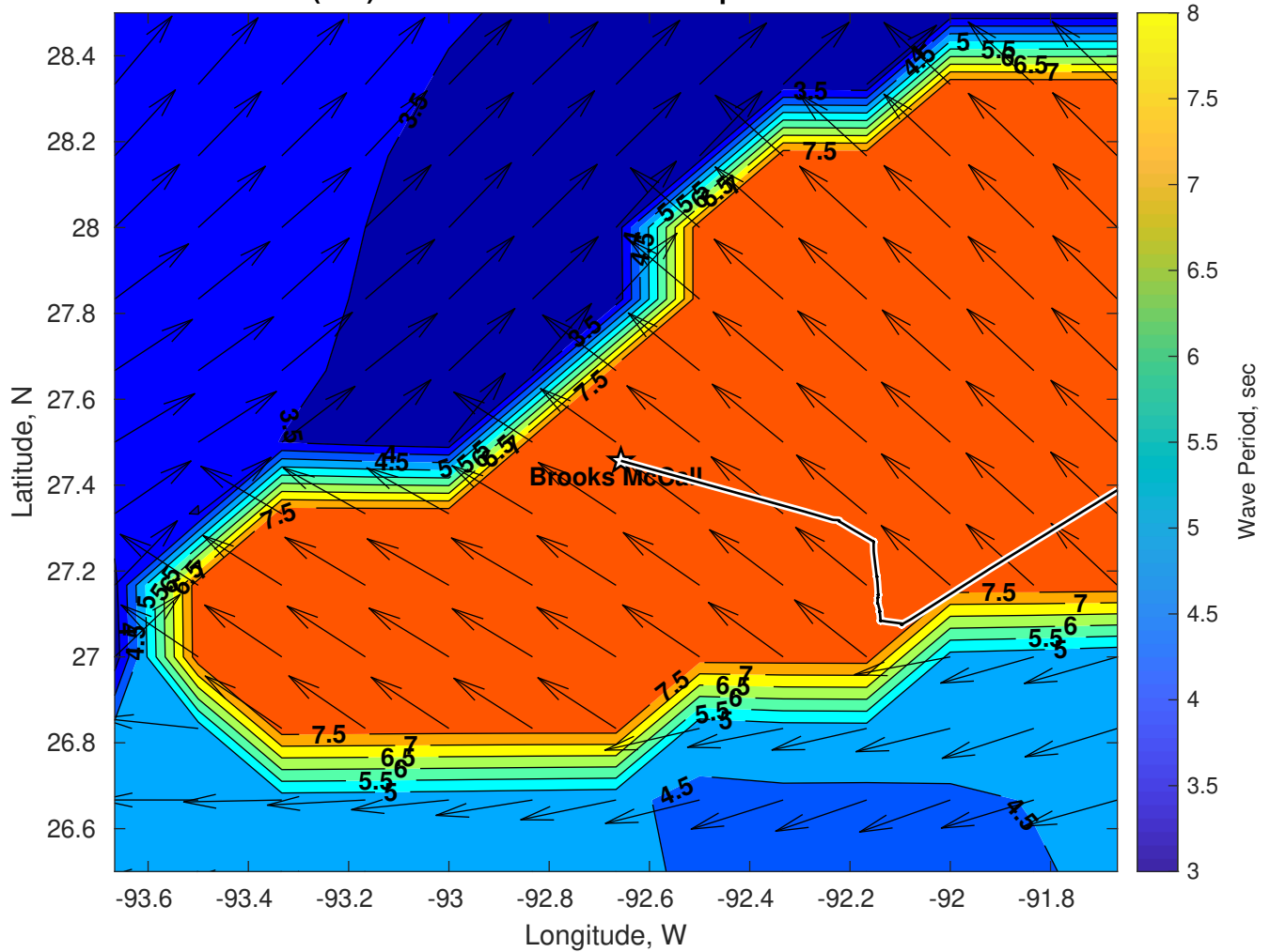
Wave Period (sec) for Brooks McCall at 10-Apr-2025 21:00:00
