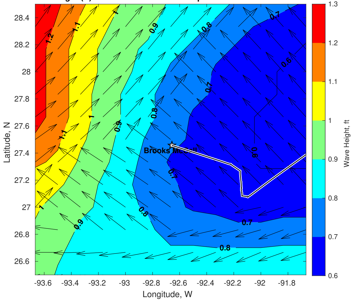
Wave Height (ft) for Brooks McCall at 10-Apr-2025 21:00:00
