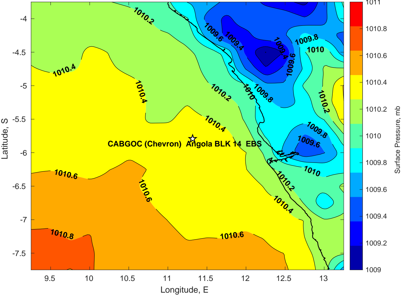
Surface Pressure (mb) for CABGOC (Chevron) Angola BLK 14 EBS at 22-Feb-2025 12:00:00
