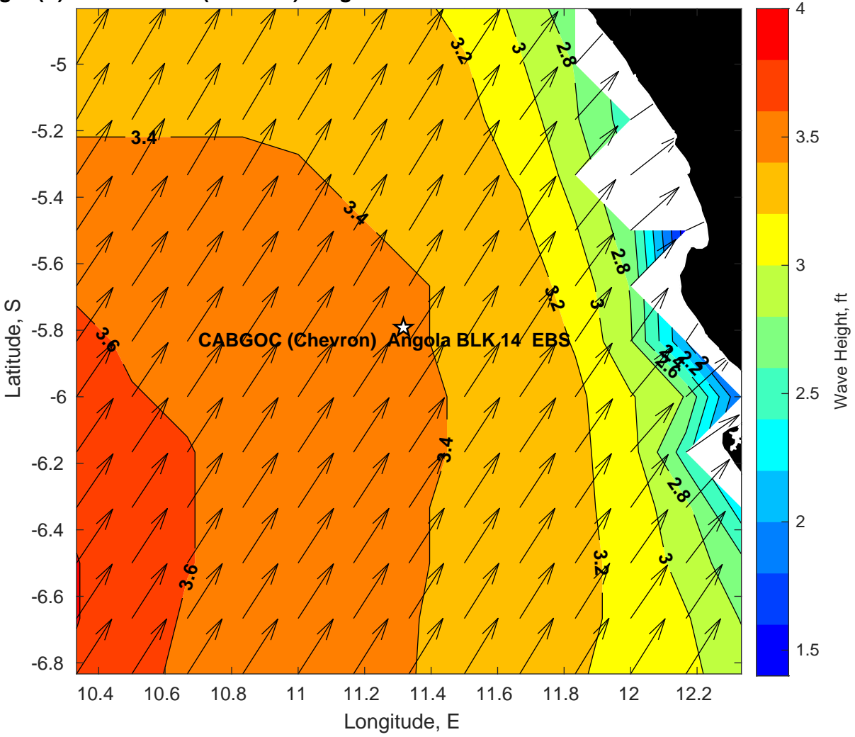
Wave Height (ft) for CABGOC (Chevron) Angola BLK 14 EBS at 22-Feb-2025 21:00:00
