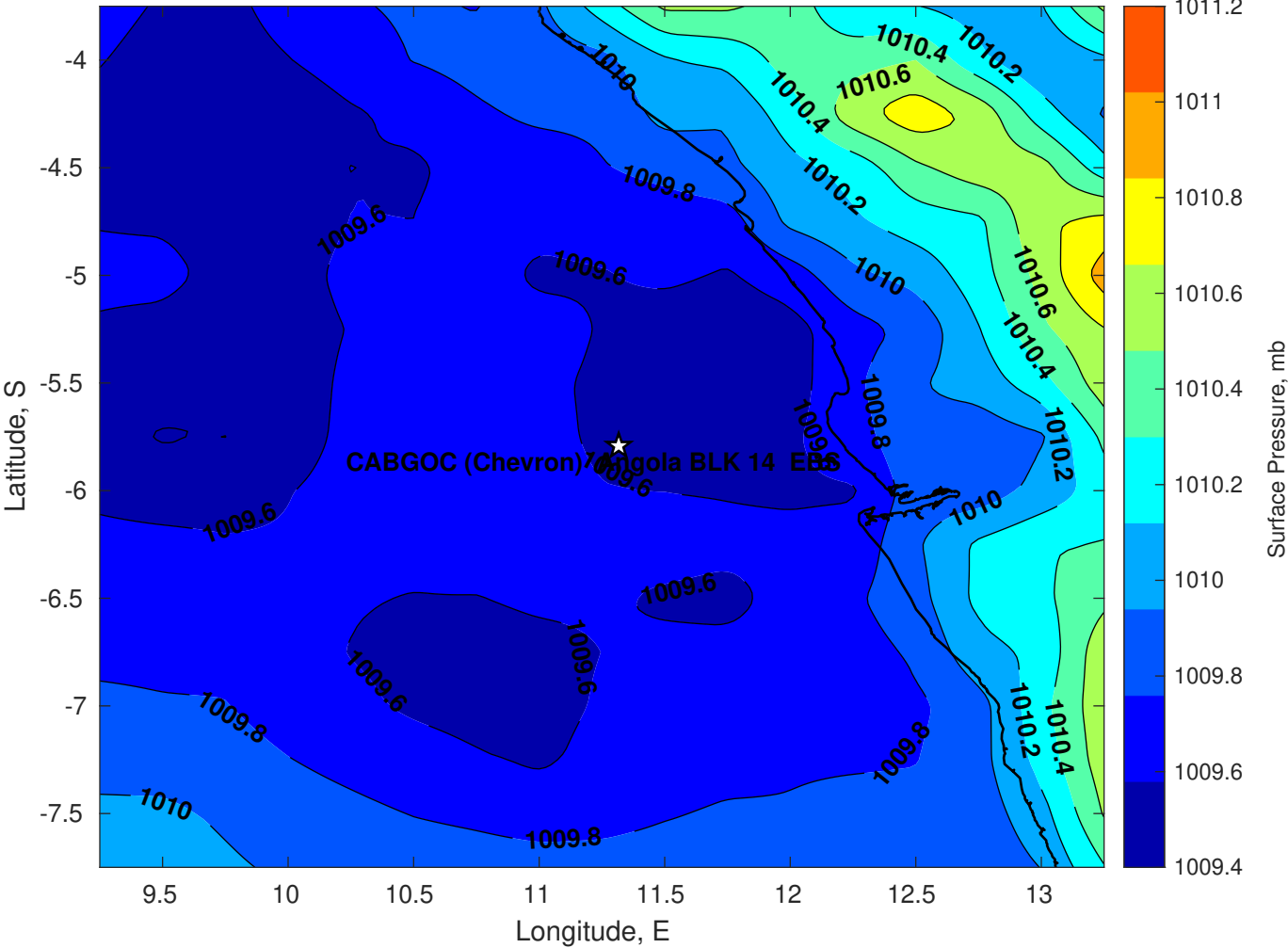
Surface Pressure (mb) for CABGOC (Chevron) Angola BLK 14 EBS at 22-Feb-2025 00:00:00
