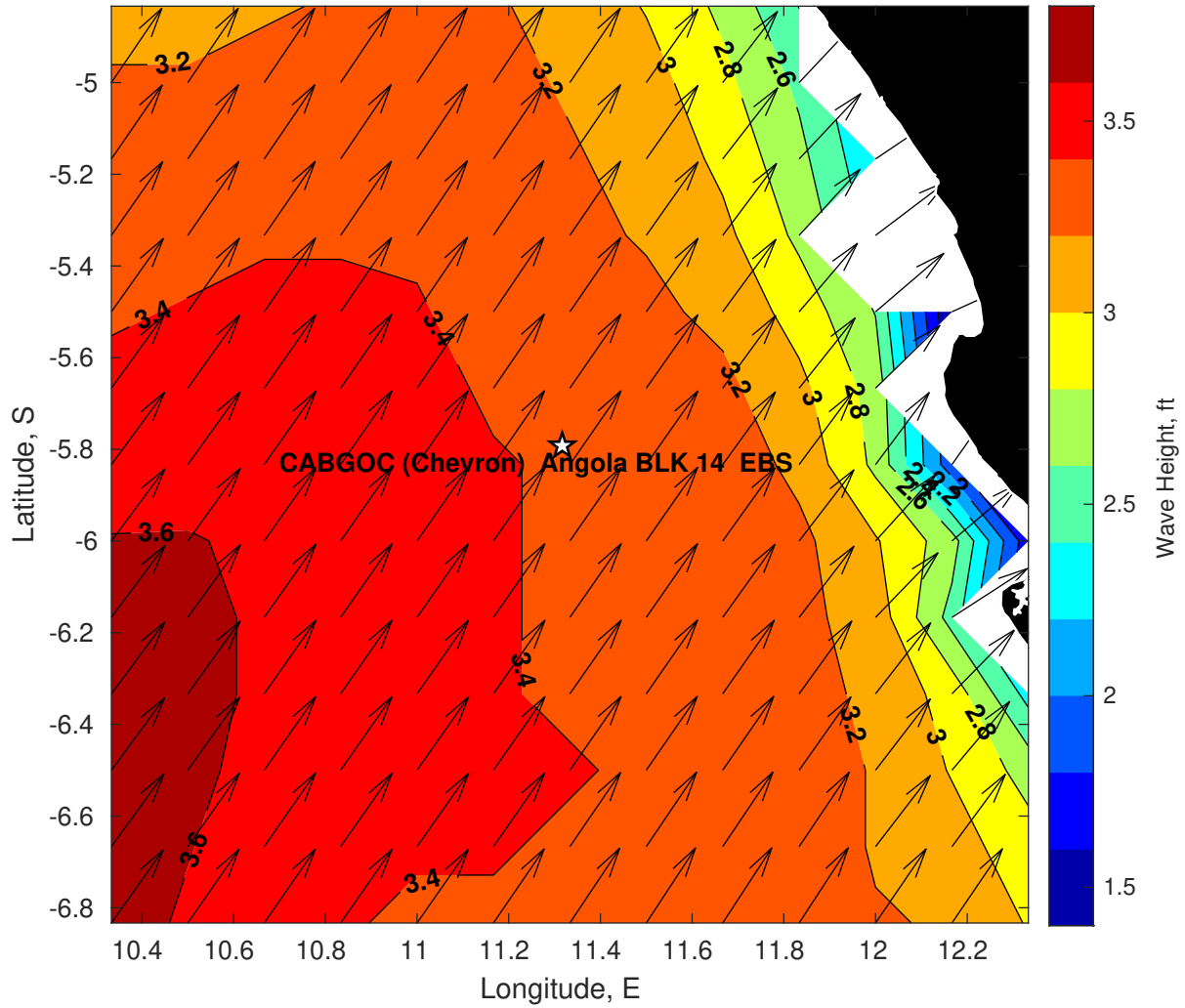
Wave Height (ft) for CABGOC (Chevron) Angola BLK 14 EBS at 22-Feb-2025 09:00:00
