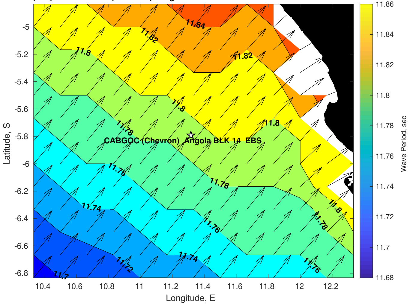
Wave Period (sec) for CABGOC (Chevron) Angola BLK 14 EBS at 22-Feb-2025 09:00:00
