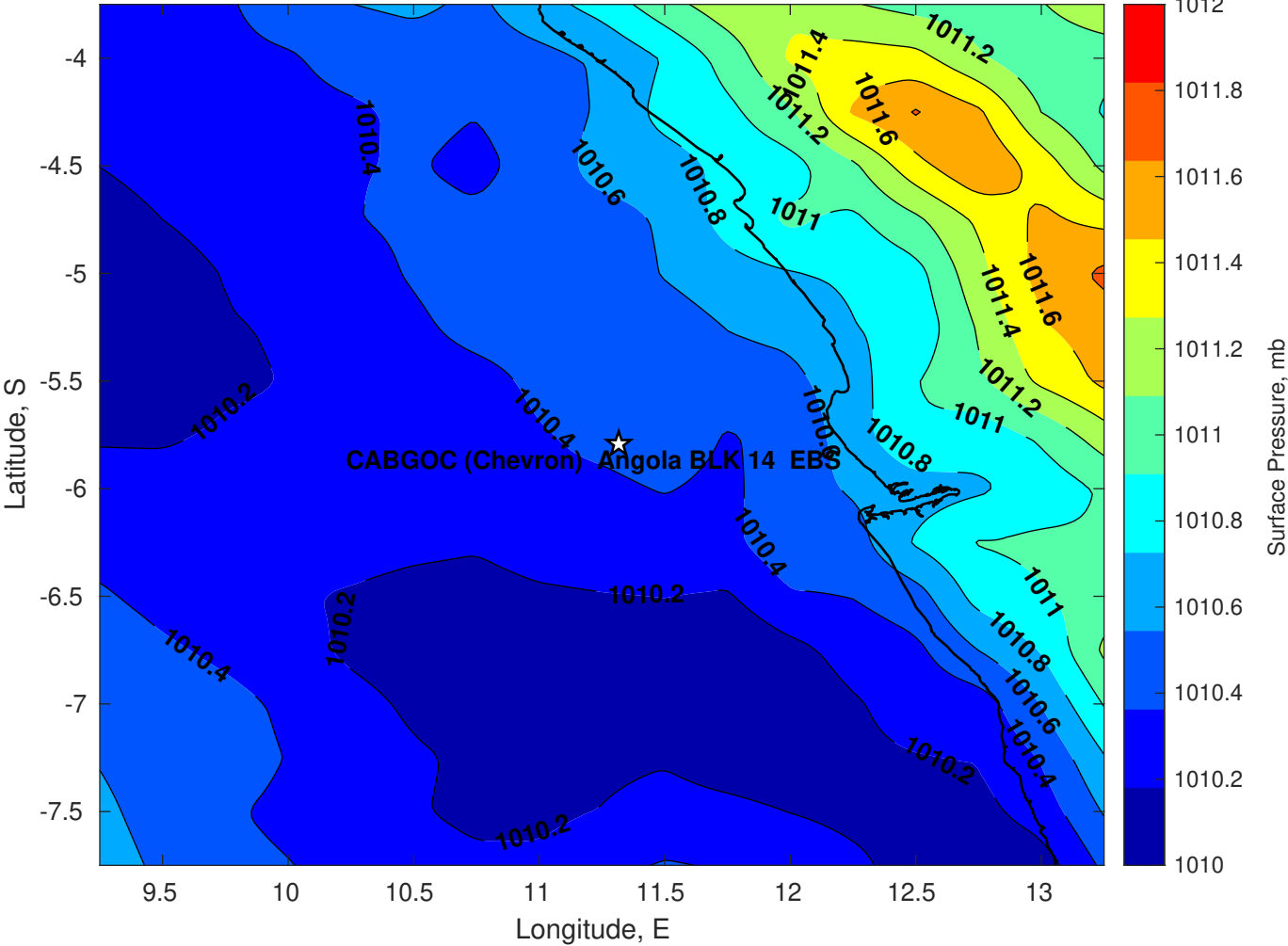
Surface Pressure (mb) for CABGOC (Chevron) Angola BLK 14 EBS at 24-Feb-2025 00:00:00
