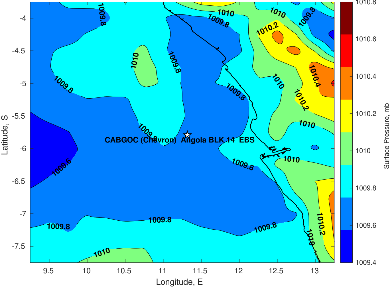
Surface Pressure (mb) for CABGOC (Chevron) Angola BLK 14 EBS at 23-Feb-2025 00:00:00
