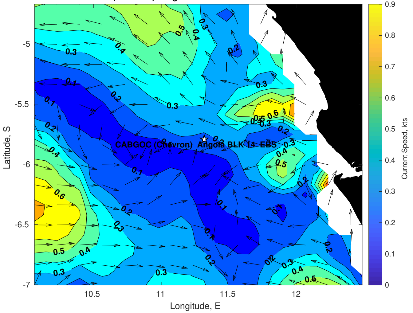
Surface Currents for CABGOC (Chevron) Angola BLK 14 EBS at 21-Feb-2025 00:00:00
