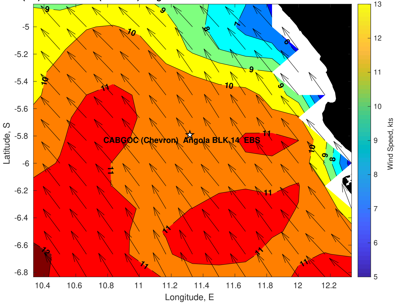
Winds (kts) for CABGOC (Chevron) Angola BLK 14 EBS at 22-Feb-2025 09:00:00
