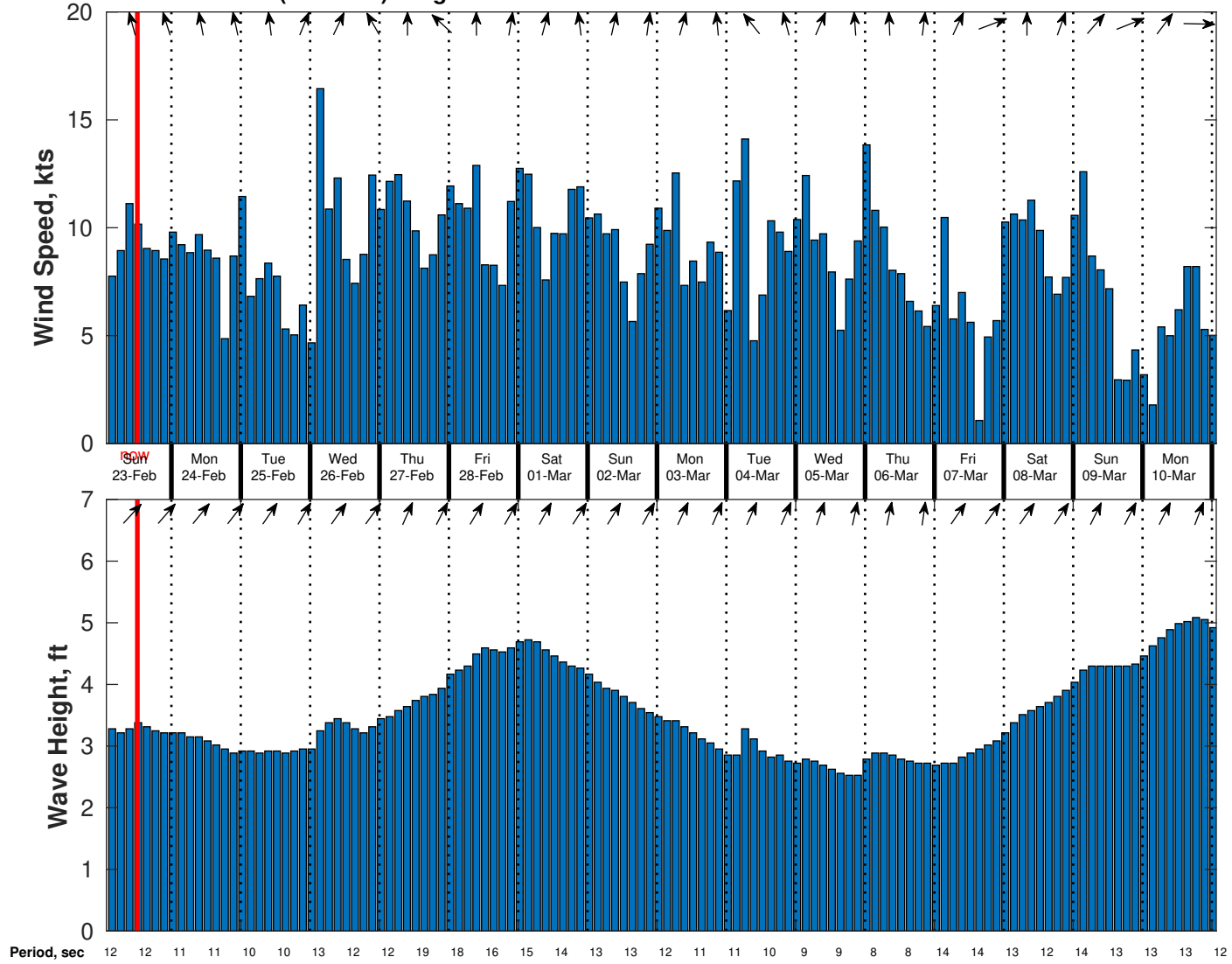
Wind & Wave Forecast for CABGOC (Chevron) Angola BLK 14 EBS from 22-Feb-2025 02:00:00 to 10-Mar-2025 02:00:00
