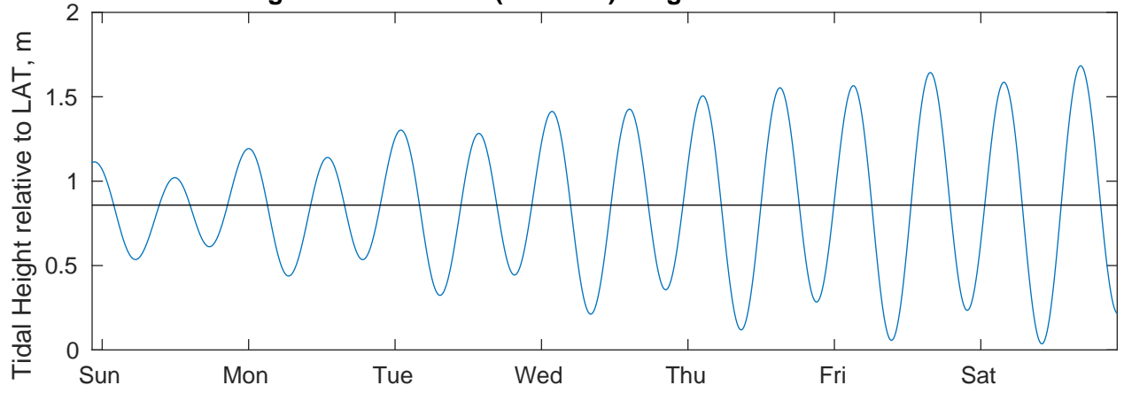
Tidal Currents and Heights for CABGOC (Chevron) Angola BLK 14 EBS at 20250222
