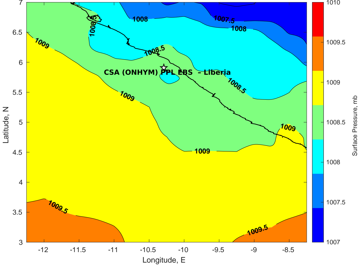
Surface Pressure (mb) for CSA (ONHYM) PPL EBS - Liberia at 22-Feb-2025 18:00:00
