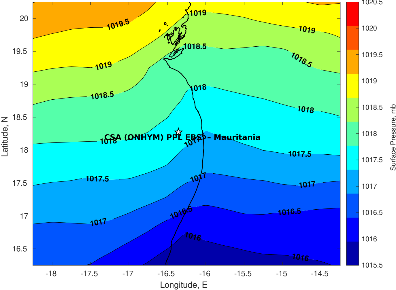
Surface Pressure (mb) for CSA (ONHYM) PPL EBS - Mauritania at 23-Feb-2025 12:00:00
