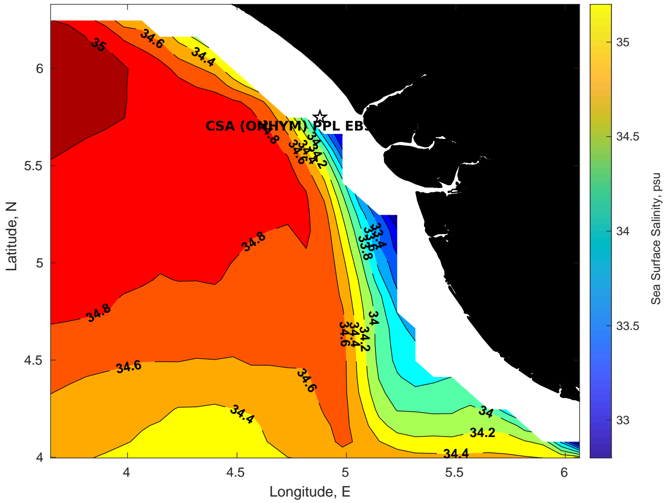
Surface Salinity for CSA (ONHYM) PPL EBS - Nigeria at 22-Feb-2025 00:00:00
