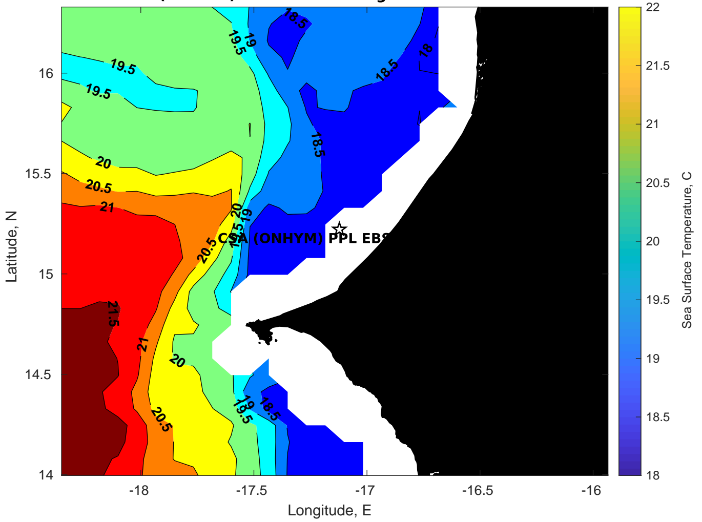
SST for CSA (ONHYM) PPL EBS - Senegal at 22-Feb-2025 00:00:00
