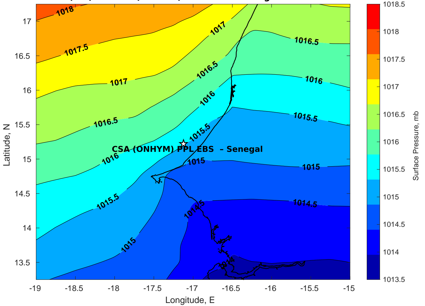
Surface Pressure (mb) for CSA (ONHYM) PPL EBS - Senegal at 24-Feb-2025 12:00:00
