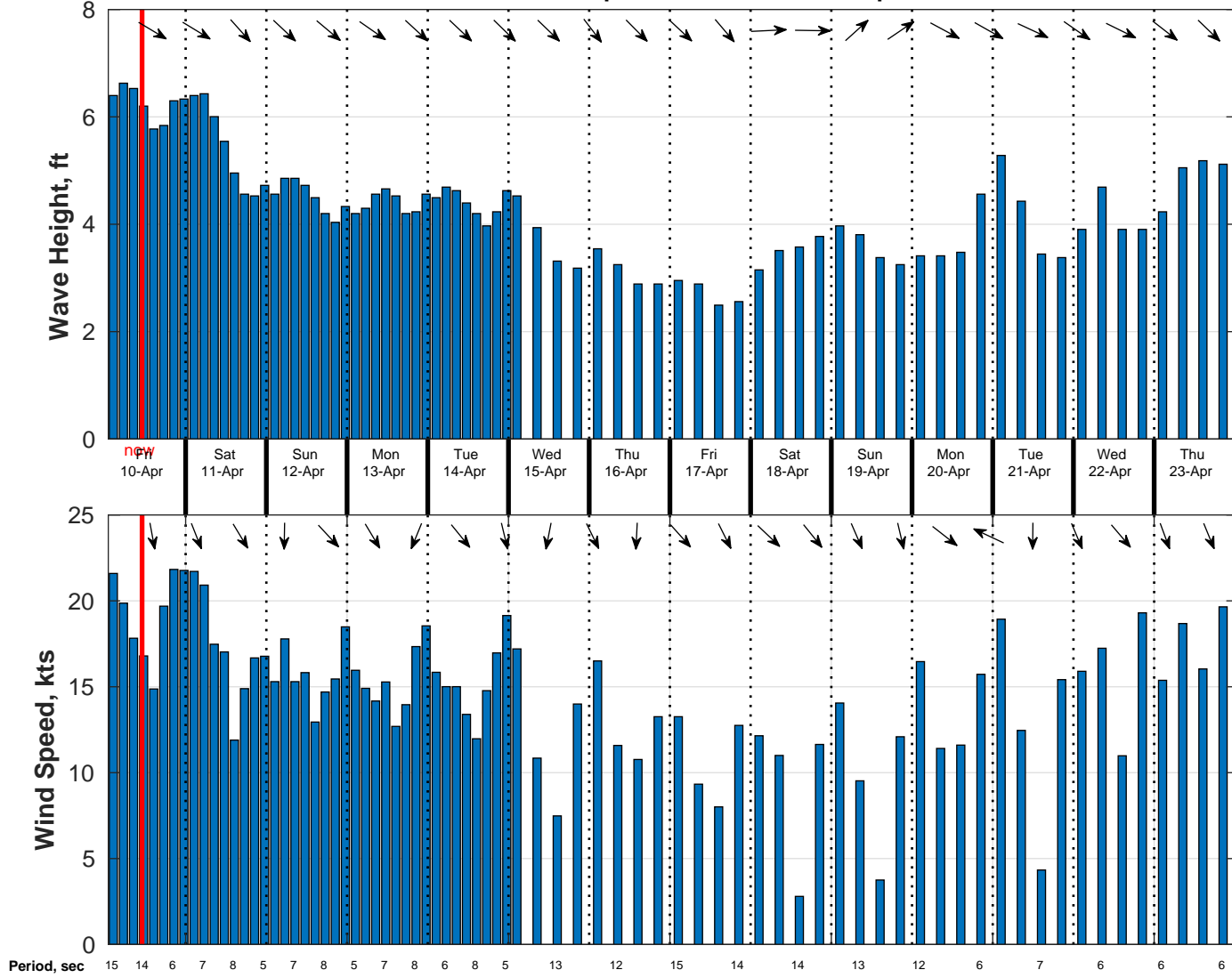
Wind & Wave Forecast for Mauritania from 09-Apr-2026 01:00:00 to 23-Apr-2026 01:00:00
