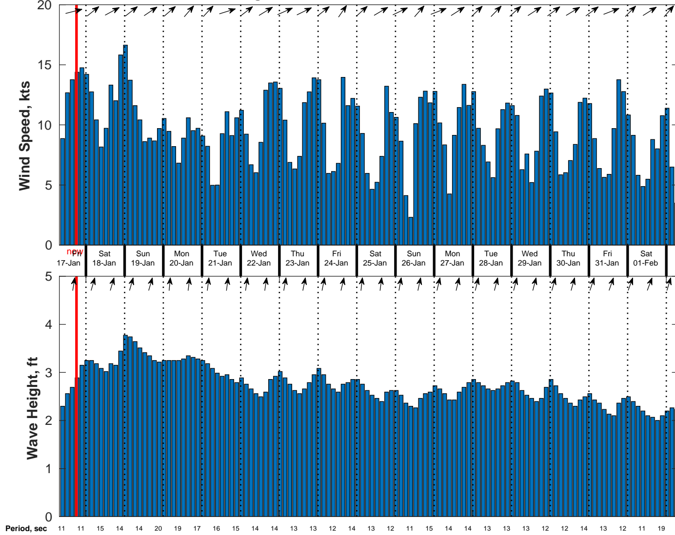
Wind & Wave Forecast for CSL Shell Nigeria from 17-Jan-2025 08:00:00 to 02-Feb-2025 08:00:00
