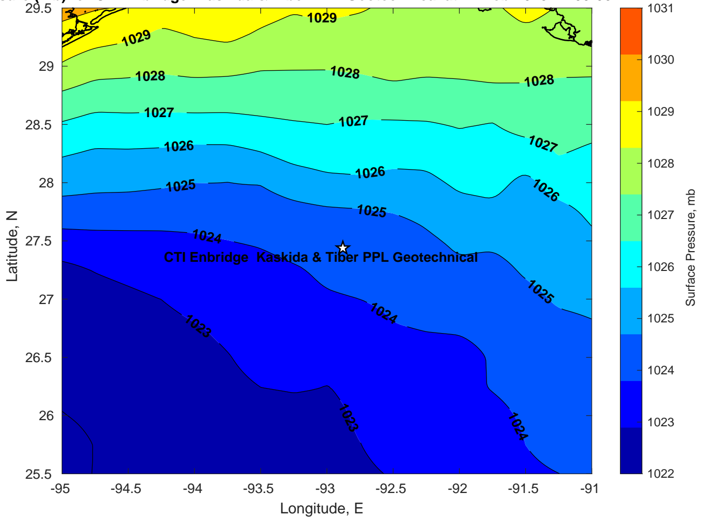
Surface Pressure (mb) for CTI Enbridge Kaskida & Tiber PPL Geotechnical at 22-Feb-2025 12:00:00
