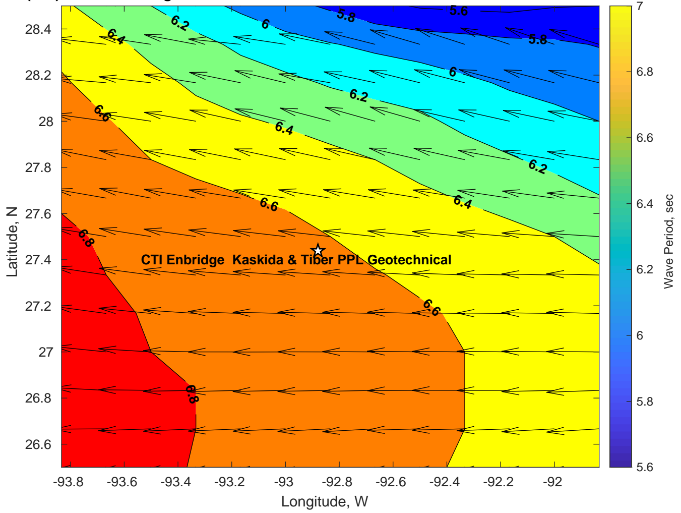
Wave Period (sec) for CTI Enbridge Kaskida & Tiber PPL Geotechnical at 22-Feb-2025 21:00:00
